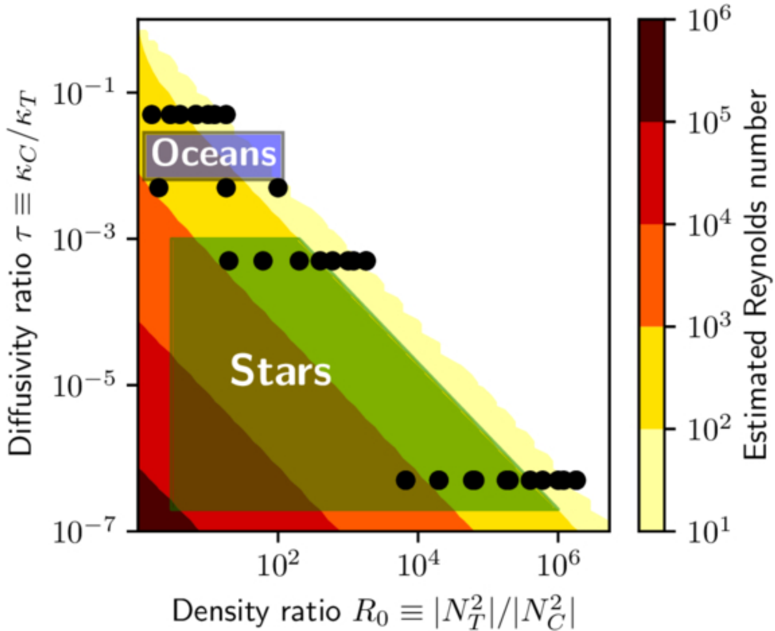
Figure 1. from Adrian E. Fraser 2026 Astrophys. J. Lett. 1001 doi:10.3847/2041-8213/ae5796 https://dx.doi.org/10.3847/2041-8213/ae5796 © 2026. The Author(s). Published by the American Astronomical Society.
