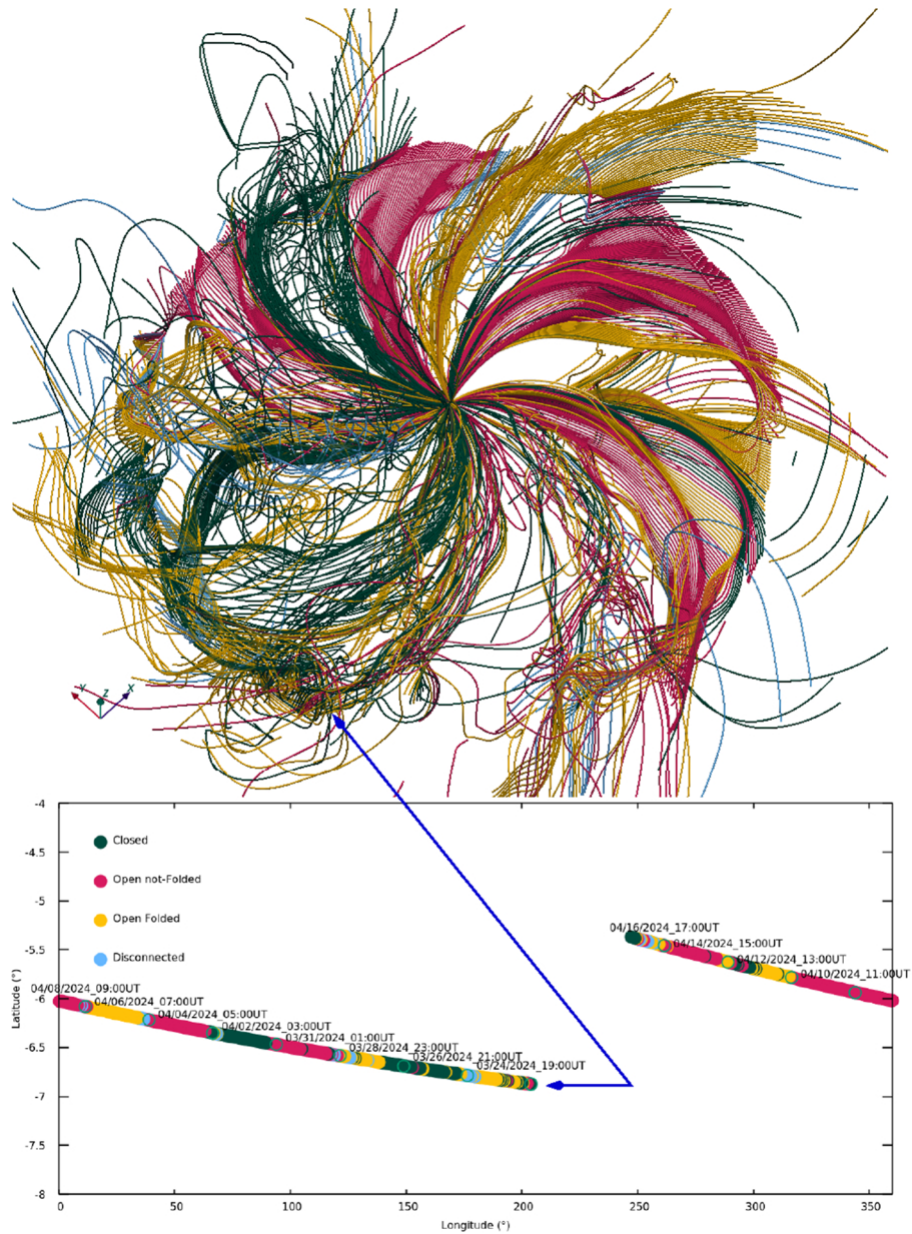
Figure 4. from Roberto Lionello et al 2026 Astrophys. J. Lett. 1001 doi:10.3847/2041-8213/ae5791 https://dx.doi.org/10.3847/2041-8213/ae5791 © 2026. The Author(s). Published by the American Astronomical Society.
