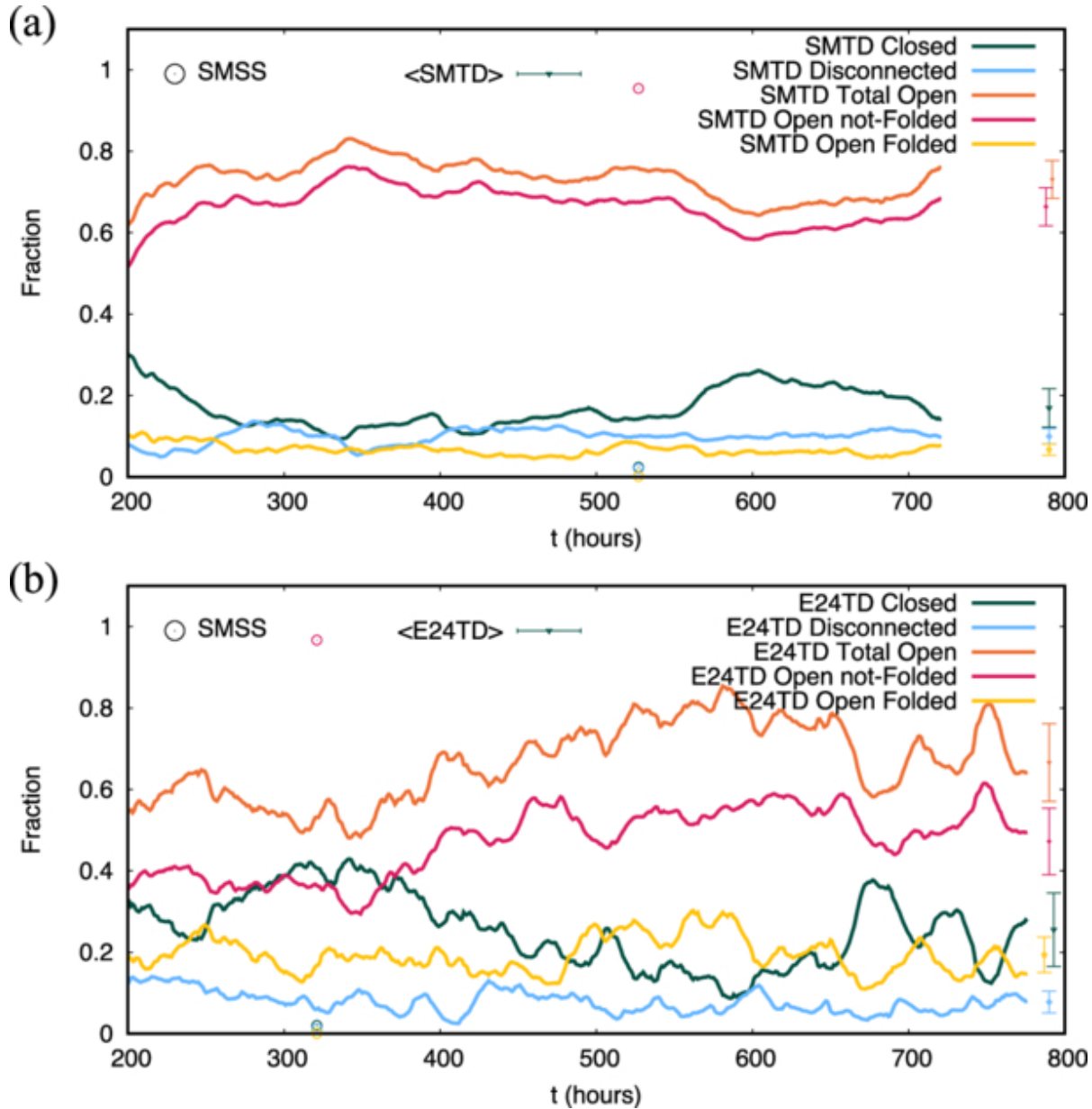
Figure 3. from Roberto Lionello et al 2026 Astrophys. J. Lett. 1001 doi:10.3847/2041-8213/ae5791 https://dx.doi.org/10.3847/2041-8213/ae5791 © 2026. The Author(s). Published by the American Astronomical Society.
