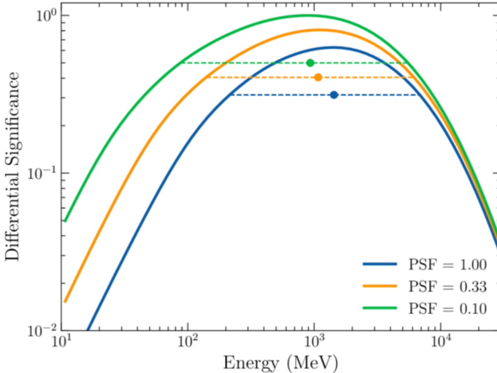
Figure 8. from M. Kerr et al 2026 Astrophys. J. Lett. 1001 doi:10.3847/2041-8213/ae570d https://dx.doi.org/10.3847/2041-8213/ae570d © 2026. The Author(s). Published by the American Astronomical Society.
