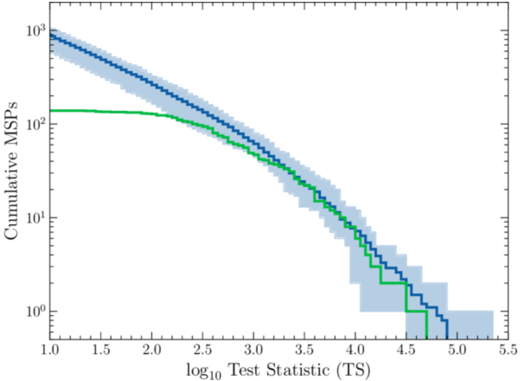
Figure 4. from M. Kerr et al 2026 Astrophys. J. Lett. 1001 doi:10.3847/2041-8213/ae570d https://dx.doi.org/10.3847/2041-8213/ae570d © 2026. The Author(s). Published by the American Astronomical Society.
