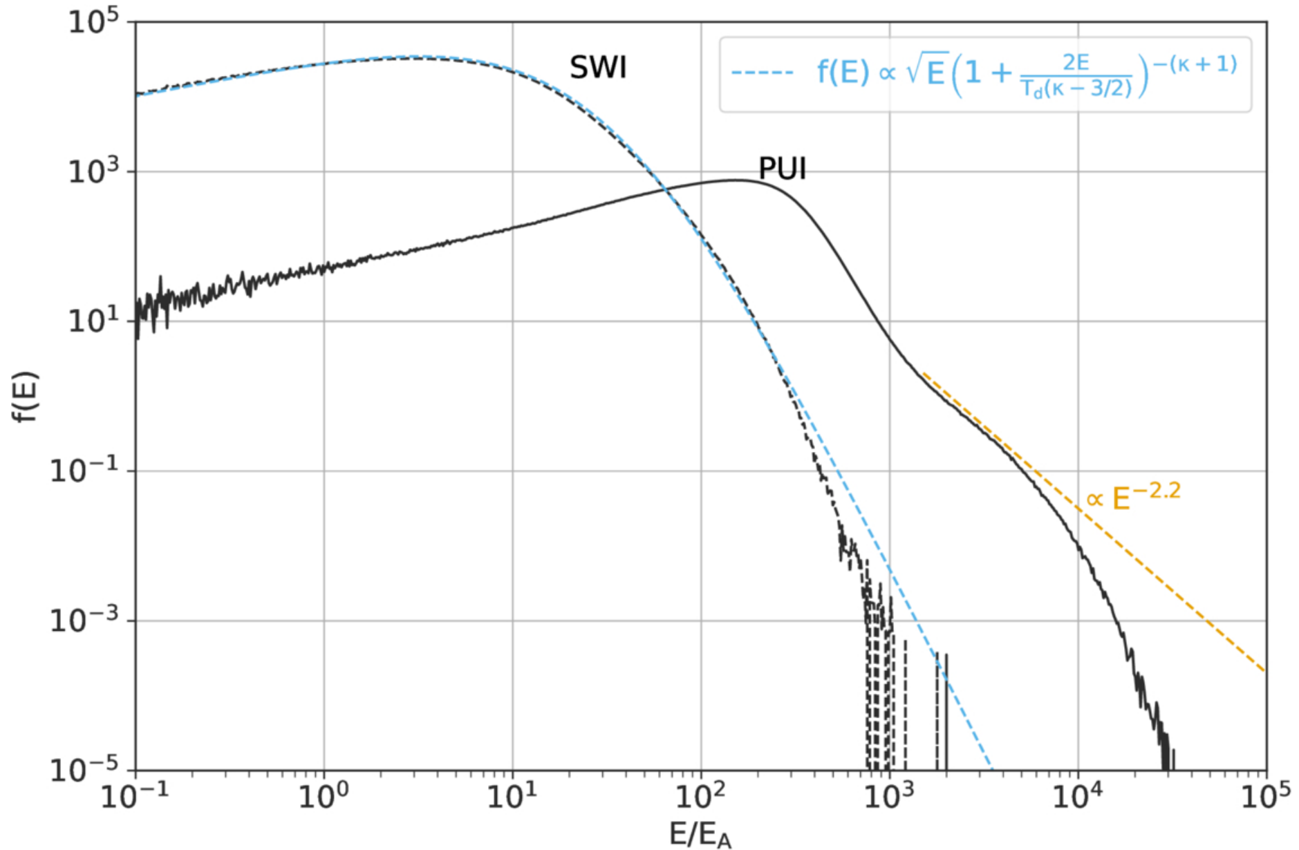
Figure 5. from Masaru Nakanotani et al 2026 Astrophys. J. Lett. 1001 doi:10.3847/2041-8213/ae5706 https://dx.doi.org/10.3847/2041-8213/ae5706 © 2026. The Author(s). Published by the American Astronomical Society.
