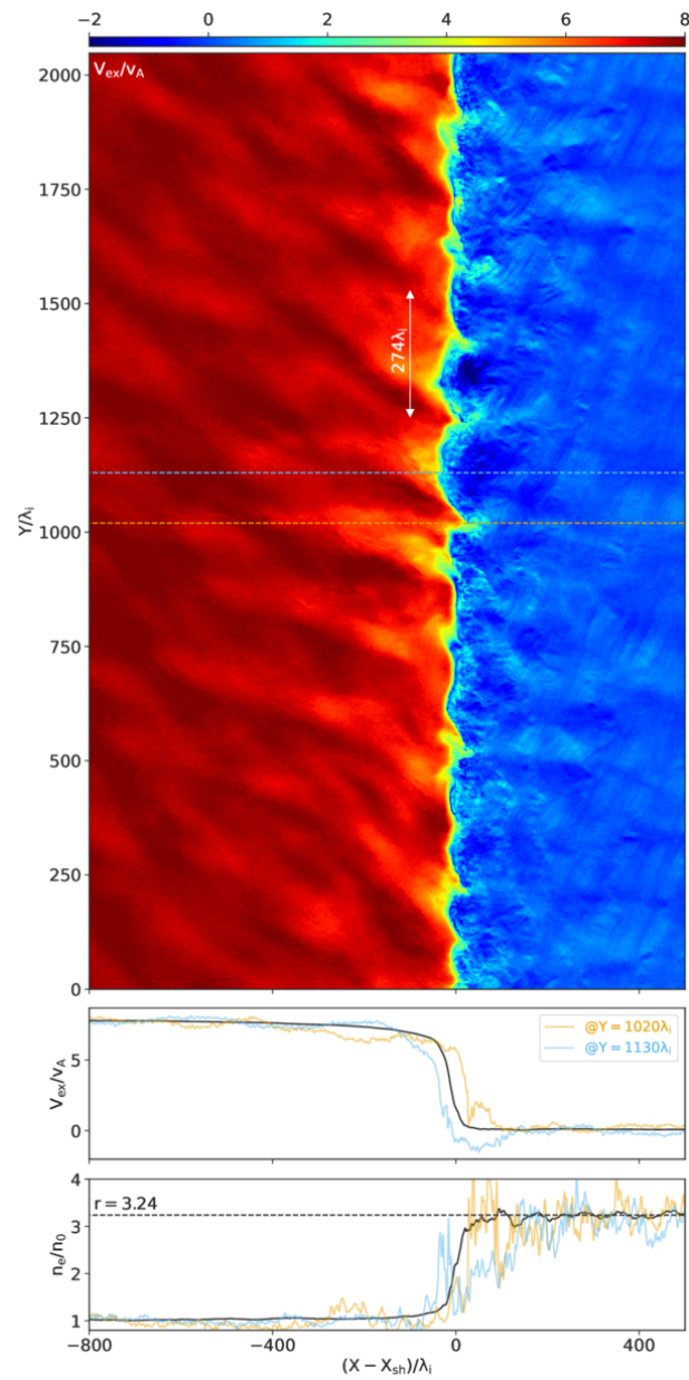
Figure 4. from Masaru Nakanotani et al 2026 Astrophys. J. Lett. 1001 doi:10.3847/2041-8213/ae5706 https://dx.doi.org/10.3847/2041-8213/ae5706 © 2026. The Author(s). Published by the American Astronomical Society.
