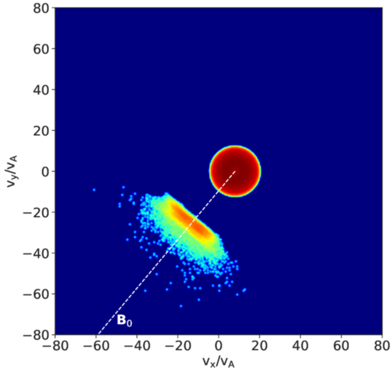
Figure 3. from Masaru Nakanotani et al 2026 Astrophys. J. Lett. 1001 doi:10.3847/2041-8213/ae5706 https://dx.doi.org/10.3847/2041-8213/ae5706 © 2026. The Author(s). Published by the American Astronomical Society.
