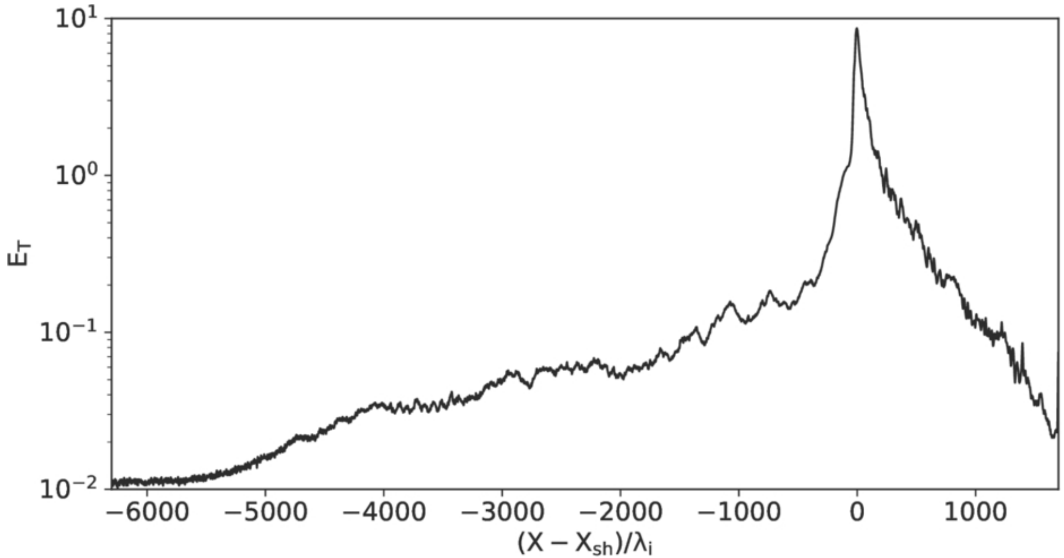
Figure 2. from Masaru Nakanotani et al 2026 Astrophys. J. Lett. 1001 doi:10.3847/2041-8213/ae5706 https://dx.doi.org/10.3847/2041-8213/ae5706 © 2026. The Author(s). Published by the American Astronomical Society.
