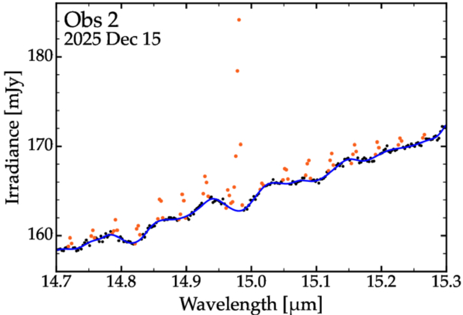
Figure 6. from Matthew Belyakov et al 2026 Astrophys. J. Lett. 1001 doi:10.3847/2041-8213/ae5700 https://dx.doi.org/10.3847/2041-8213/ae5700 © 2026. The Author(s). Published by the American Astronomical Society.
