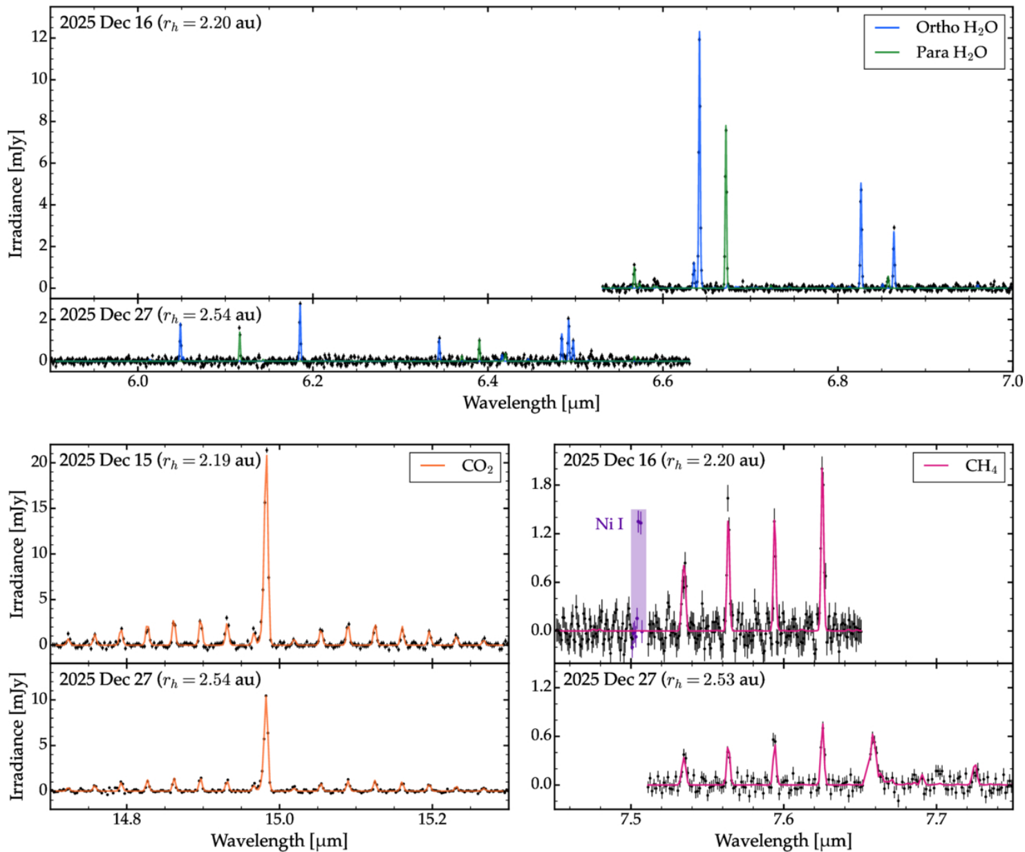
Figure 2. from Matthew Belyakov et al 2026 Astrophys. J. Lett. 1001 doi:10.3847/2041-8213/ae5700 https://dx.doi.org/10.3847/2041-8213/ae5700 © 2026. The Author(s). Published by the American Astronomical Society.
