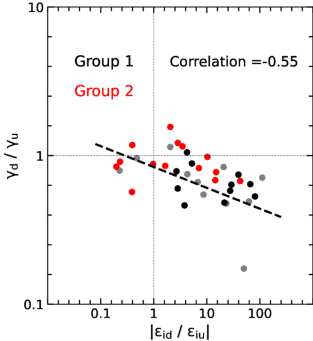
Figure 5. from Yiming Jiao et al 2026 Astrophys. J. Lett. 1001 doi:10.3847/2041-8213/ae561c https://dx.doi.org/10.3847/2041-8213/ae561c © 2026. The Author(s). Published by the American Astronomical Society.
