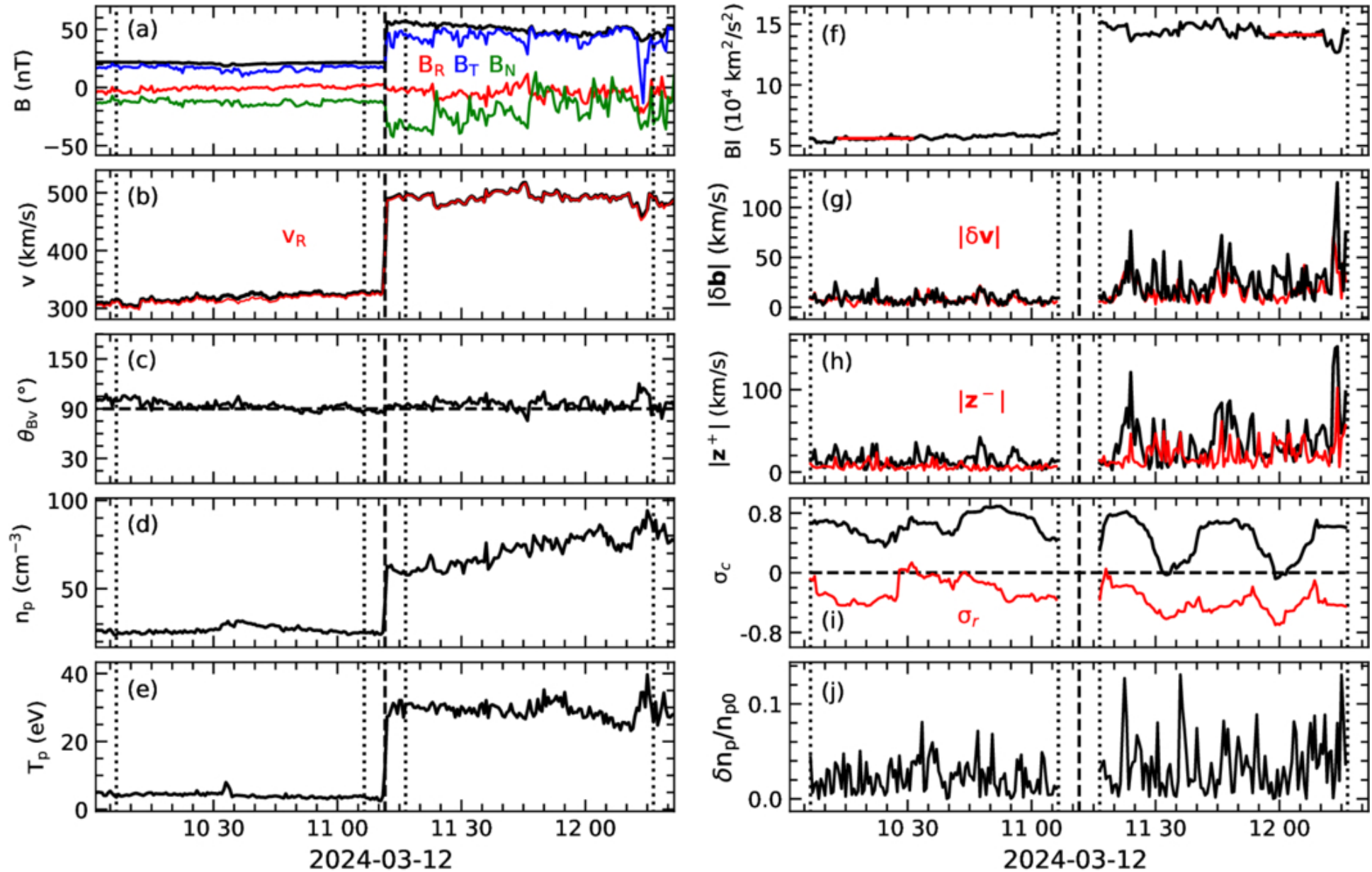
Figure 1. from Yiming Jiao et al 2026 Astrophys. J. Lett. 1001 doi:10.3847/2041-8213/ae561c https://dx.doi.org/10.3847/2041-8213/ae561c © 2026. The Author(s). Published by the American Astronomical Society.
