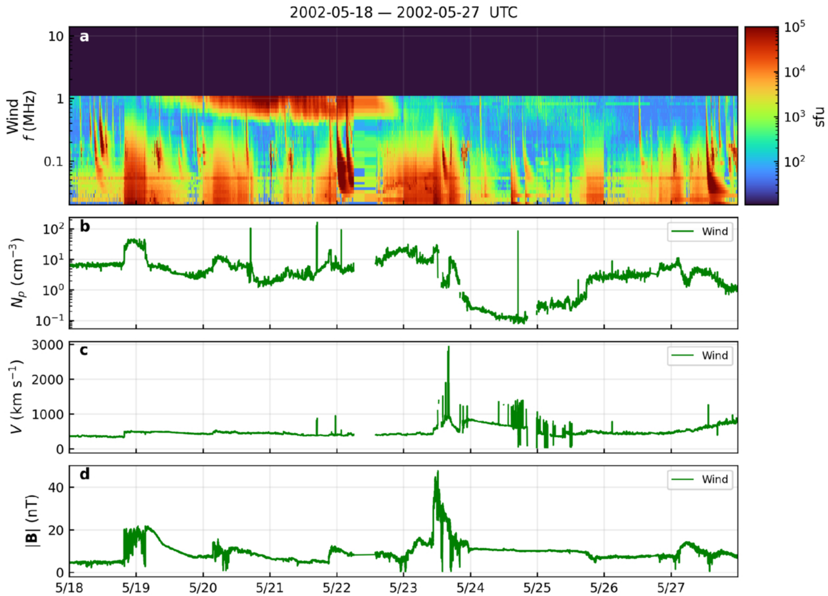
Figure 9. from Vratislav Krupar et al 2026 Astrophys. J. Lett. 1003 doi:10.3847/2041-8213/ae5537 https://dx.doi.org/10.3847/2041-8213/ae5537 © 2026. The Author(s). Published by the American Astronomical Society.
