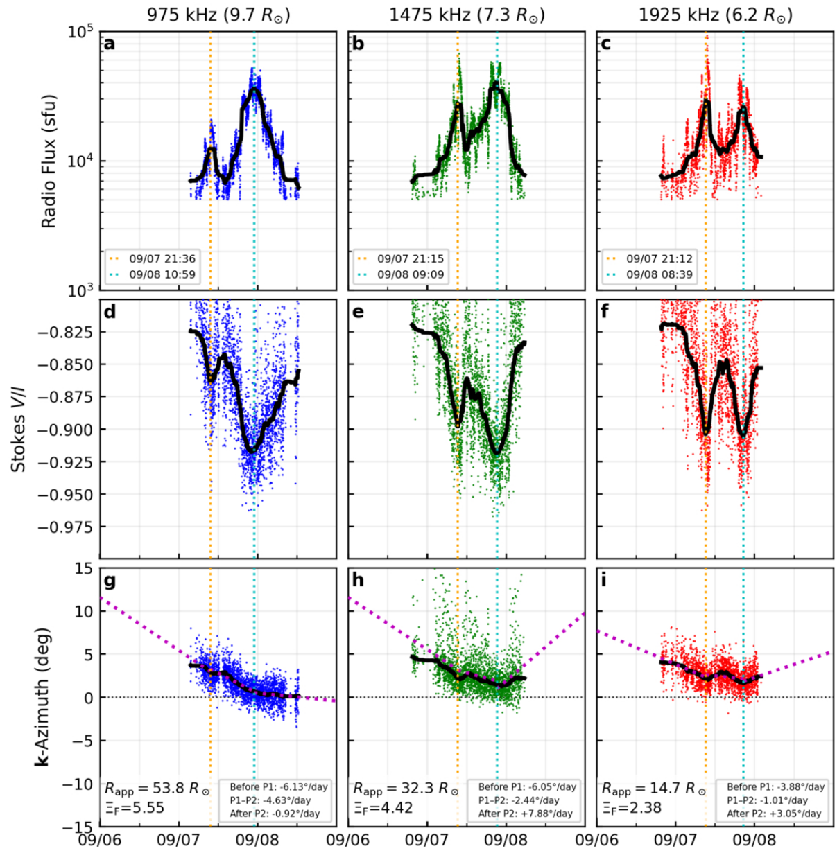
Figure 6. from Vratislav Krupar et al 2026 Astrophys. J. Lett. 1003 doi:10.3847/2041-8213/ae5537 https://dx.doi.org/10.3847/2041-8213/ae5537 © 2026. The Author(s). Published by the American Astronomical Society.
