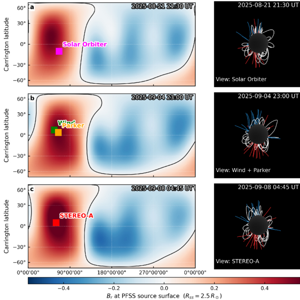
Figure 4. from Vratislav Krupar et al 2026 Astrophys. J. Lett. 1003 doi:10.3847/2041-8213/ae5537 https://dx.doi.org/10.3847/2041-8213/ae5537 © 2026. The Author(s). Published by the American Astronomical Society.
