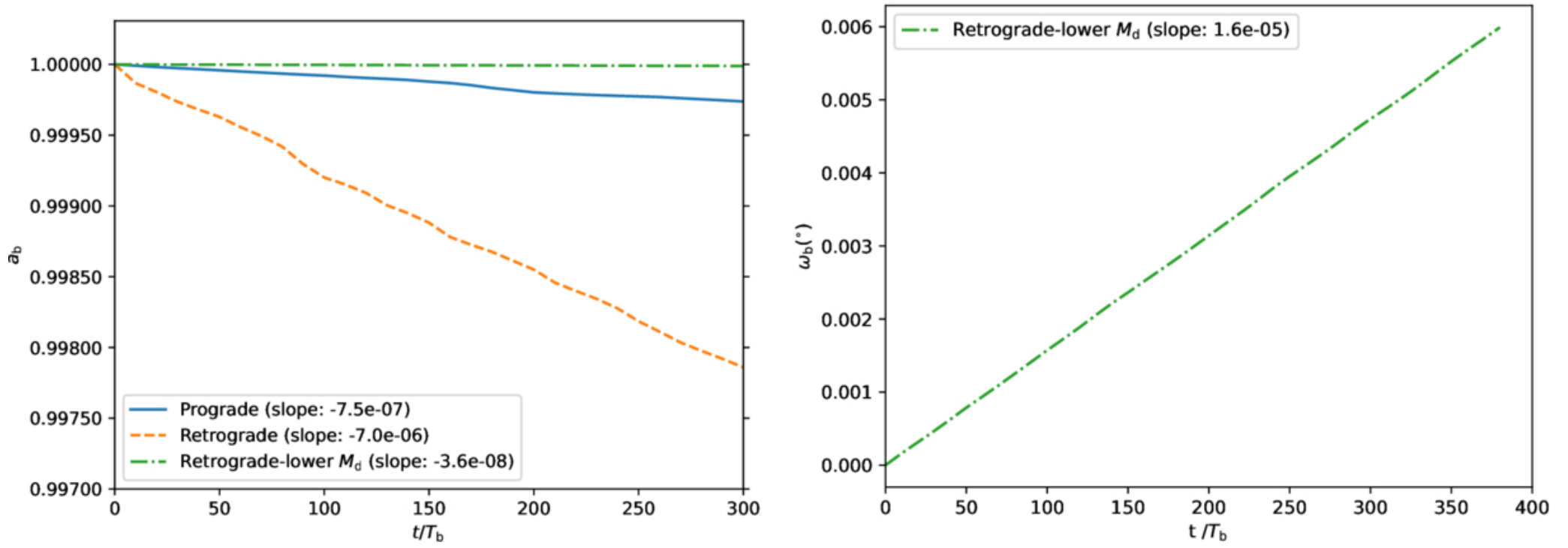
Figure 8. from Cheng Chen et al 2026 Astrophys. J. Lett. 1001 doi:10.3847/2041-8213/ae5534 https://dx.doi.org/10.3847/2041-8213/ae5534 © 2026. The Author(s). Published by the American Astronomical Society.
