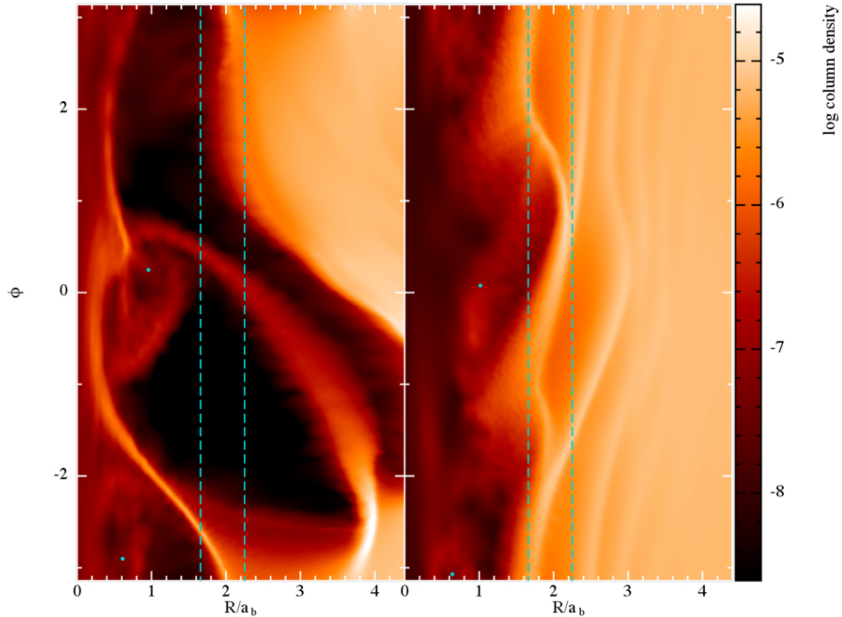
Figure 6. from Cheng Chen et al 2026 Astrophys. J. Lett. 1001 doi:10.3847/2041-8213/ae5534 https://dx.doi.org/10.3847/2041-8213/ae5534 © 2026. The Author(s). Published by the American Astronomical Society.
