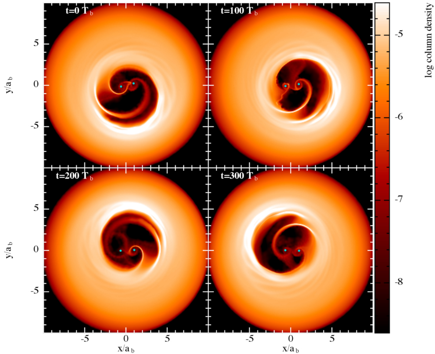
Figure 2. from Cheng Chen et al 2026 Astrophys. J. Lett. 1001 doi:10.3847/2041-8213/ae5534 https://dx.doi.org/10.3847/2041-8213/ae5534 © 2026. The Author(s). Published by the American Astronomical Society.
