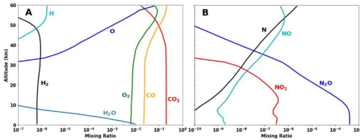
Figure 5. from Kensei Kobayashi et al 2026 Astrophys. J. Lett. 1002 doi:10.3847/2041-8213/ae5491 https://dx.doi.org/10.3847/2041-8213/ae5491 © 2026. The Author(s). Published by the American Astronomical Society.
