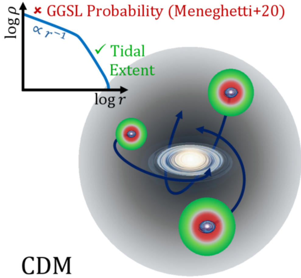
Figure 4. from Priyamvada Natarajan et al 2026 Astrophys. J. Lett. 1001 doi:10.3847/2041-8213/ae53ea https://dx.doi.org/10.3847/2041-8213/ae53ea © 2026. The Author(s). Published by the American Astronomical Society.
