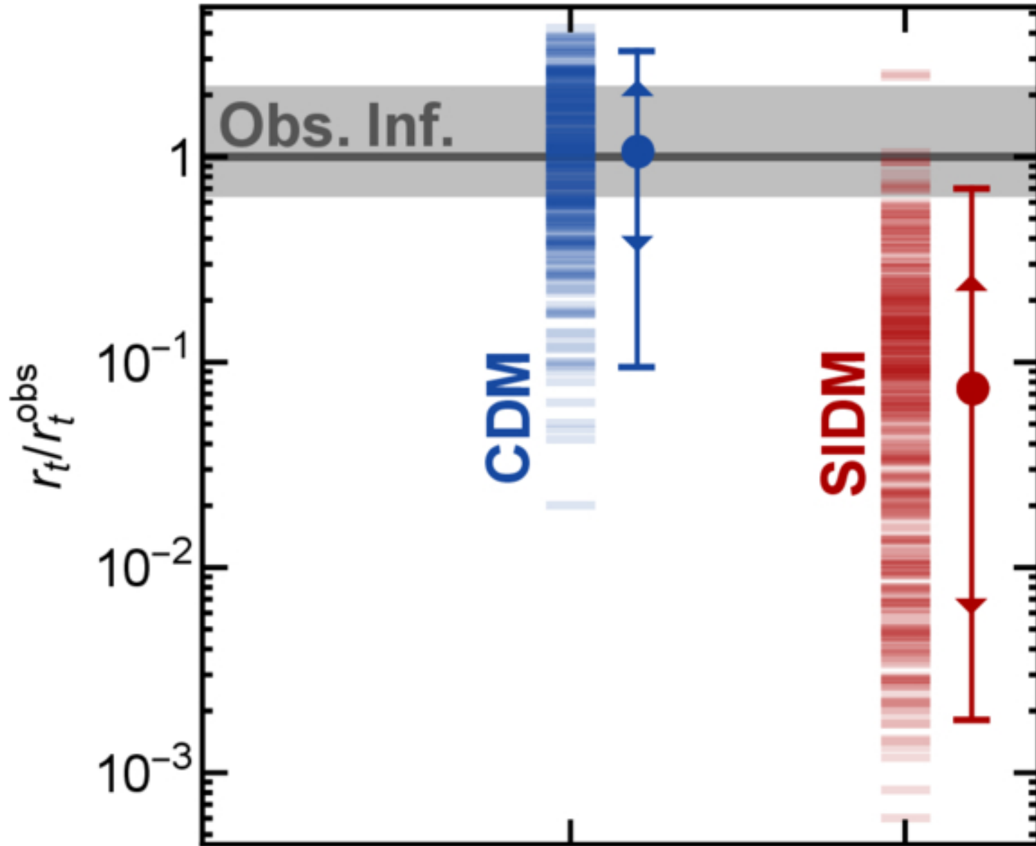
Figure 3. from Priyamvada Natarajan et al 2026 Astrophys. J. Lett. 1001 doi:10.3847/2041-8213/ae53ea https://dx.doi.org/10.3847/2041-8213/ae53ea © 2026. The Author(s). Published by the American Astronomical Society.
