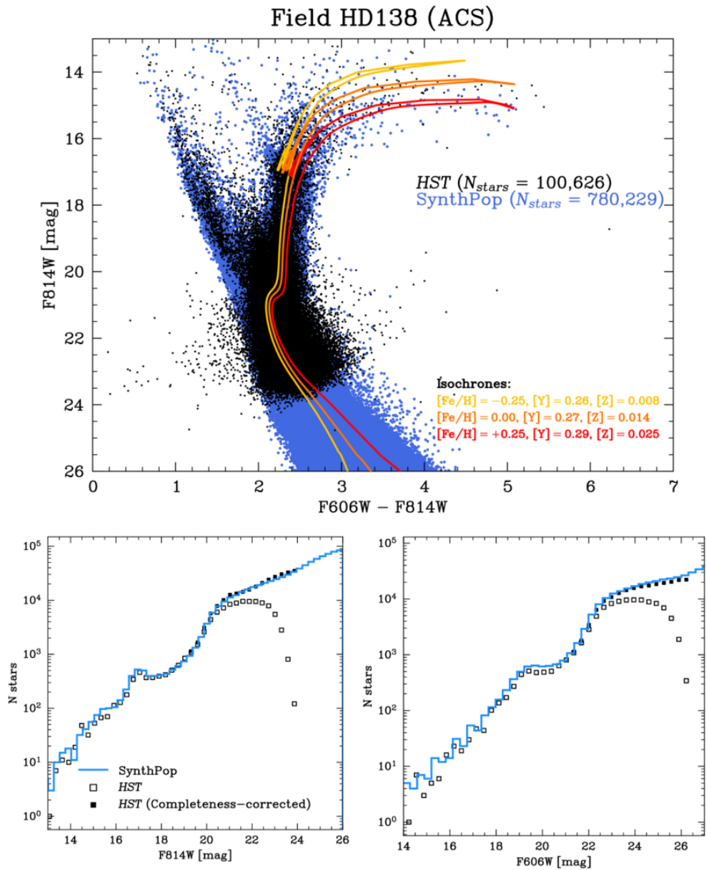
Figure 5. from Sean K. Terry et al 2026 Astrophys. J. Lett. 1003 doi:10.3847/2041-8213/ae53e8 https://dx.doi.org/10.3847/2041-8213/ae53e8 © 2026. The Author(s). Published by the American Astronomical Society.
