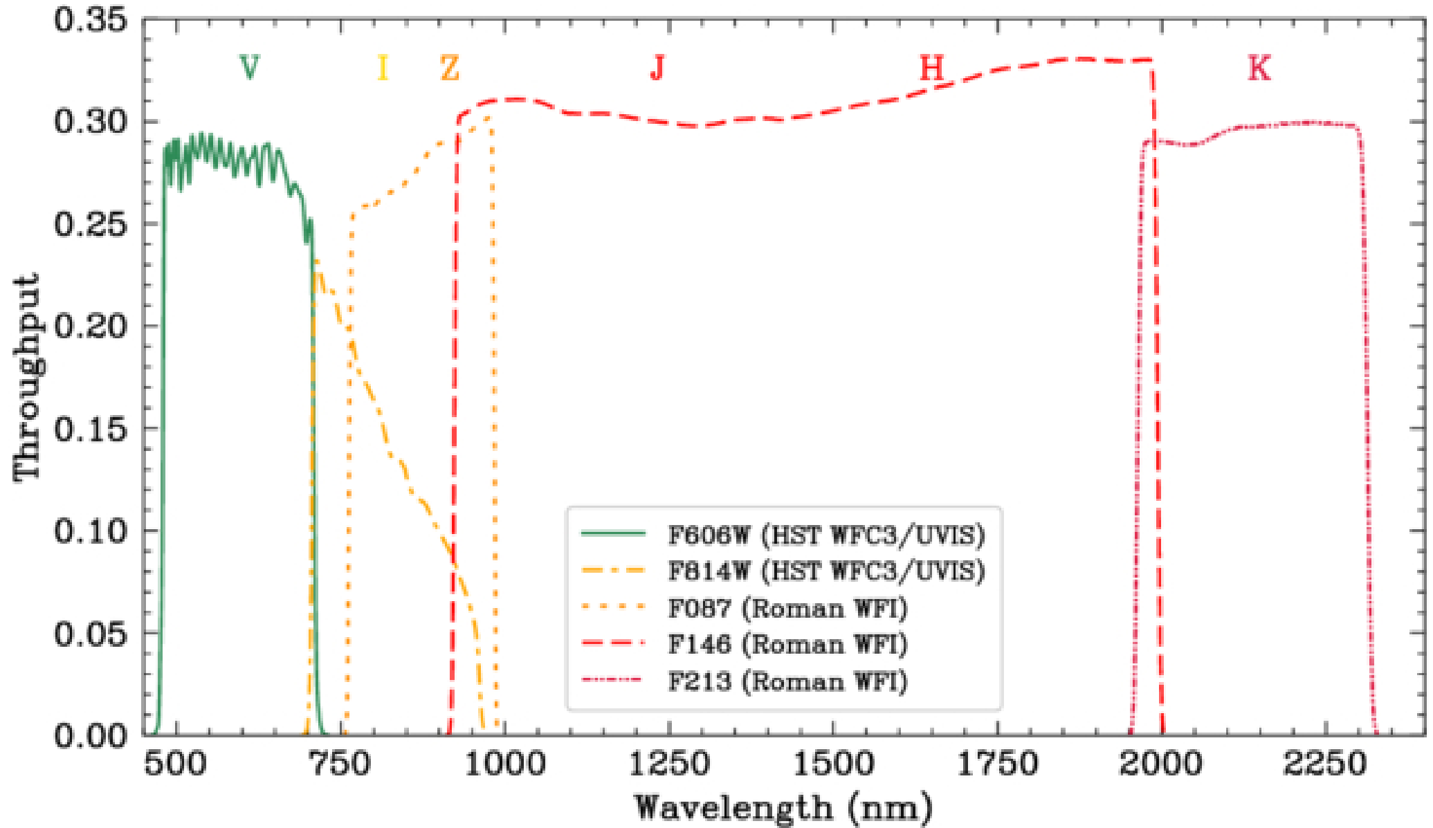
Figure 2. from Sean K. Terry et al 2026 Astrophys. J. Lett. 1003 doi:10.3847/2041-8213/ae53e8 https://dx.doi.org/10.3847/2041-8213/ae53e8 © 2026. The Author(s). Published by the American Astronomical Society.
