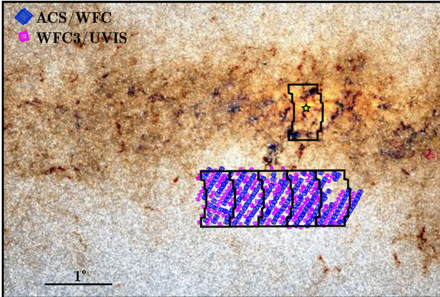
Figure 1. from Sean K. Terry et al 2026 Astrophys. J. Lett. 1003 doi:10.3847/2041-8213/ae53e8 https://dx.doi.org/10.3847/2041-8213/ae53e8 © 2026. The Author(s). Published by the American Astronomical Society.
