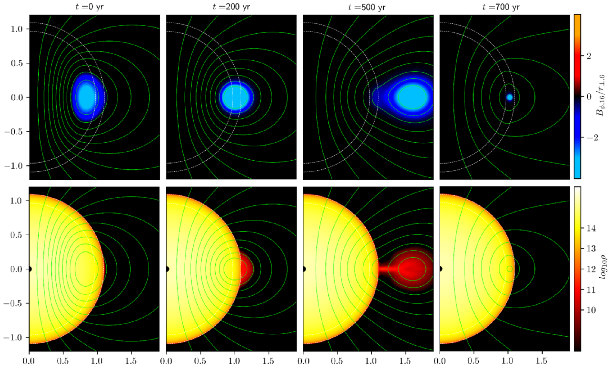
Figure 2. from Ashley Bransgrove et al 2026 Astrophys. J. Lett. 1001 doi:10.3847/2041-8213/ae50f2 https://dx.doi.org/10.3847/2041-8213/ae50f2 © 2026. The Author(s). Published by the American Astronomical Society.
