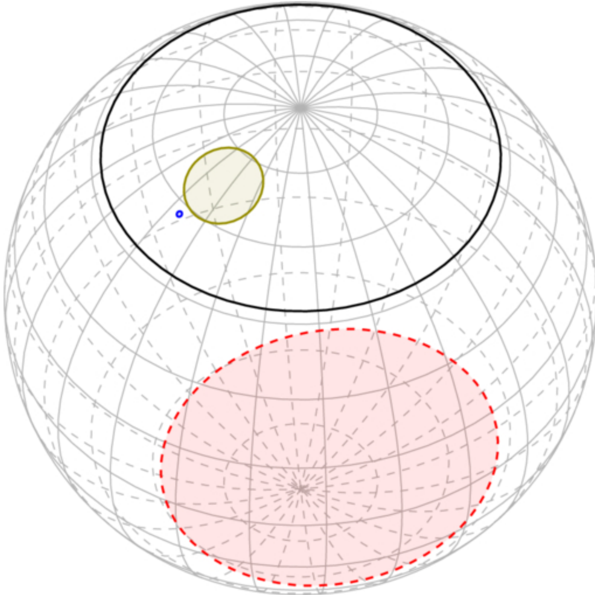
Figure 2. from M. C. Miller et al 2026 Astrophys. J. Lett. 1000 doi:10.3847/2041-8213/ae5057 https://dx.doi.org/10.3847/2041-8213/ae5057 © 2026. The Author(s). Published by the American Astronomical Society.
