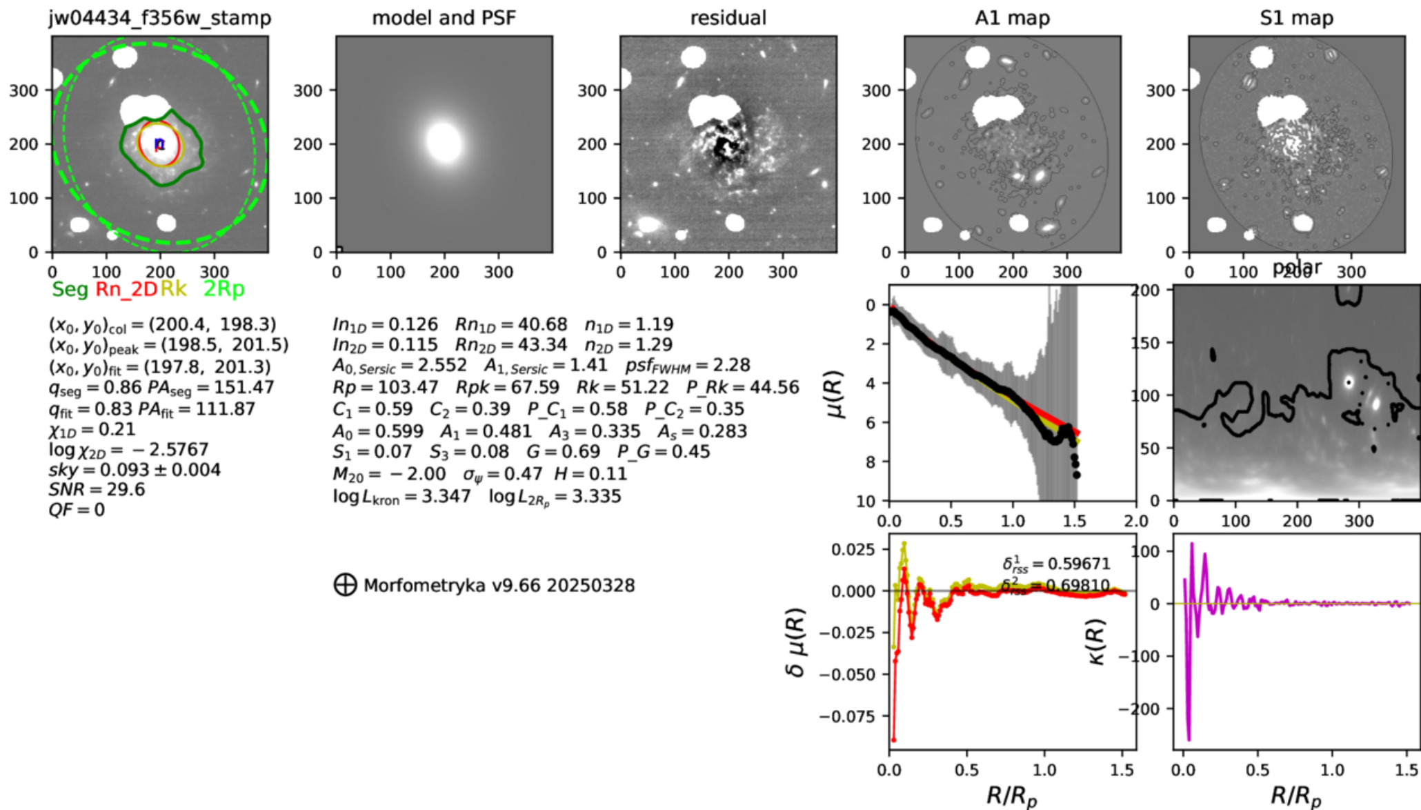
Figure A3. from Clecio R. Bom et al 2026 Astrophys. J. Lett. 1001 doi:10.3847/2041-8213/ae4fbe https://dx.doi.org/10.3847/2041-8213/ae4fbe © 2026. The Author(s). Published by the American Astronomical Society.
