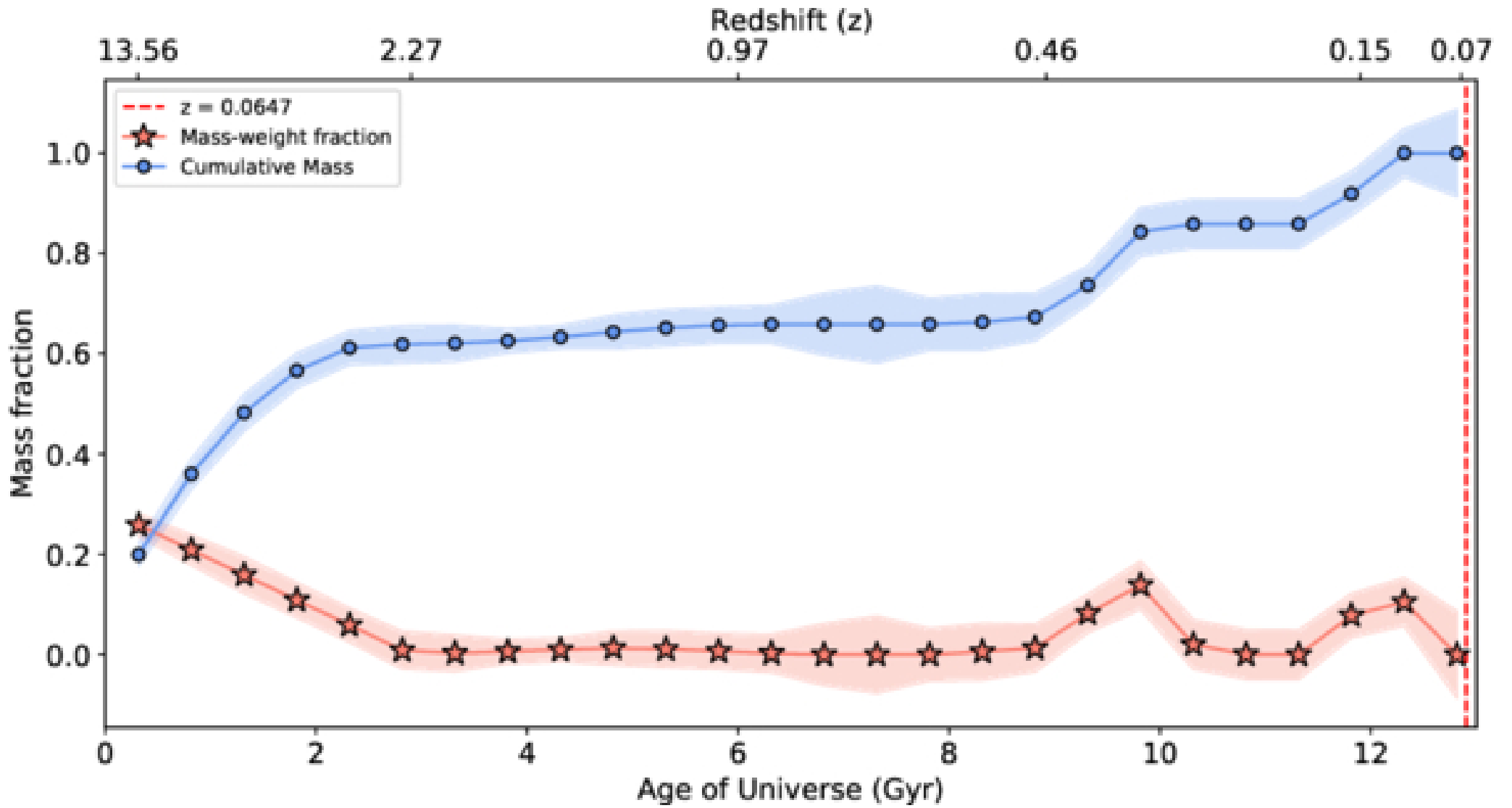
Figure D1. from Clecio R. Bom et al 2026 Astrophys. J. Lett. 1001 doi:10.3847/2041-8213/ae4fbe https://dx.doi.org/10.3847/2041-8213/ae4fbe © 2026. The Author(s). Published by the American Astronomical Society.
