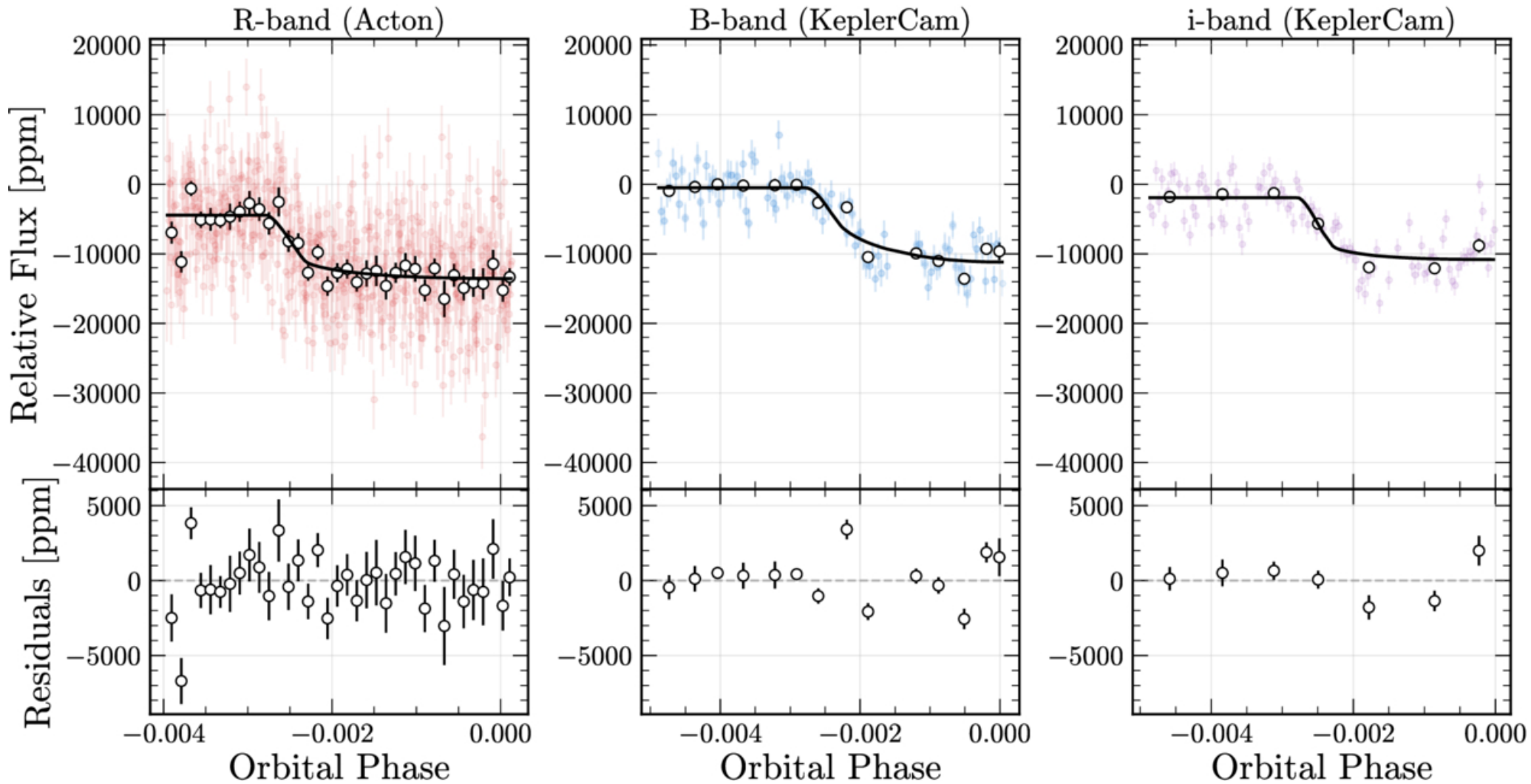
Figure 9. from Jéa Adams Redai et al 2026 Astrophys. J. Lett. 1002 doi:10.3847/2041-8213/ae4ec5 https://dx.doi.org/10.3847/2041-8213/ae4ec5 © 2026. The Author(s). Published by the American Astronomical Society.
