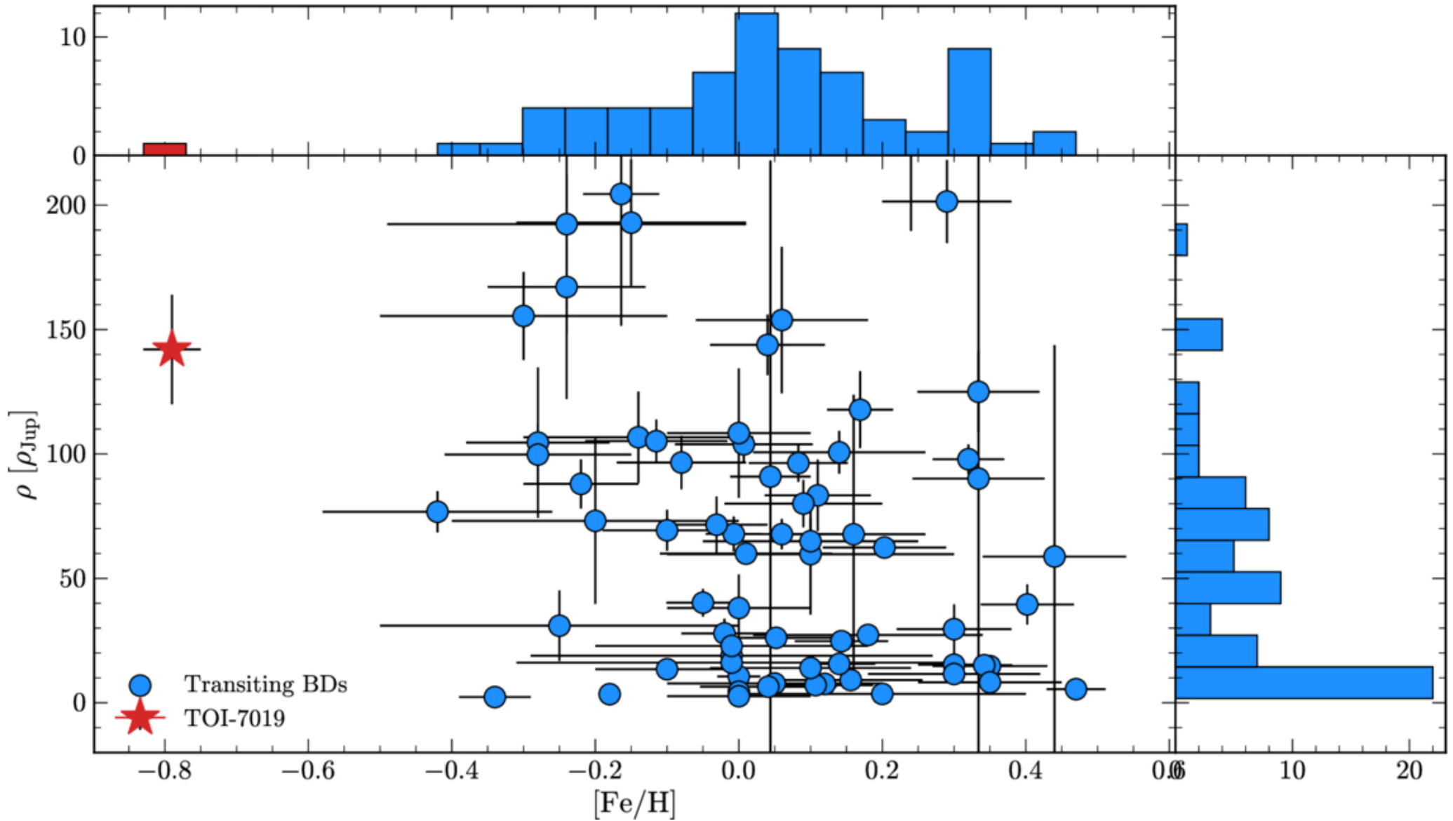
Figure 7. from Jéa Adams Redai et al 2026 Astrophys. J. Lett. 1002 doi:10.3847/2041-8213/ae4ec5 https://dx.doi.org/10.3847/2041-8213/ae4ec5 © 2026. The Author(s). Published by the American Astronomical Society.
