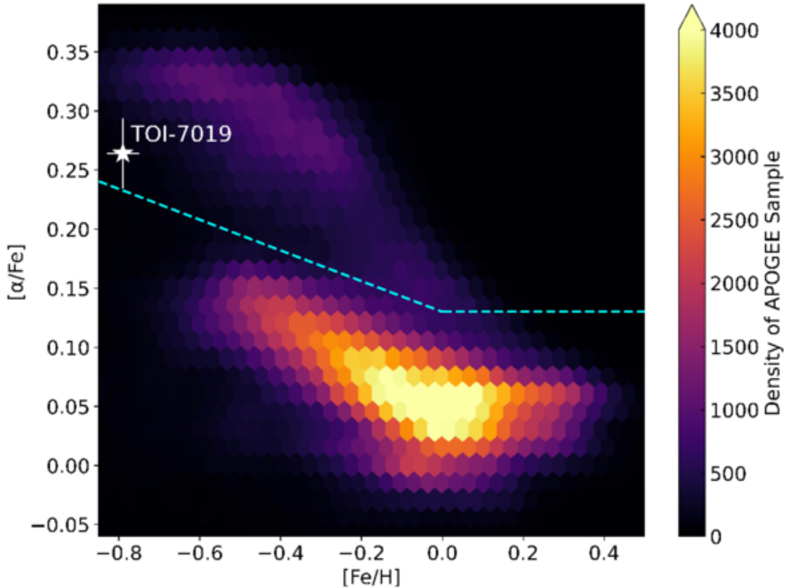
Figure 3. from Jéa Adams Redai et al 2026 Astrophys. J. Lett. 1002 doi:10.3847/2041-8213/ae4ec5 https://dx.doi.org/10.3847/2041-8213/ae4ec5 © 2026. The Author(s). Published by the American Astronomical Society.
