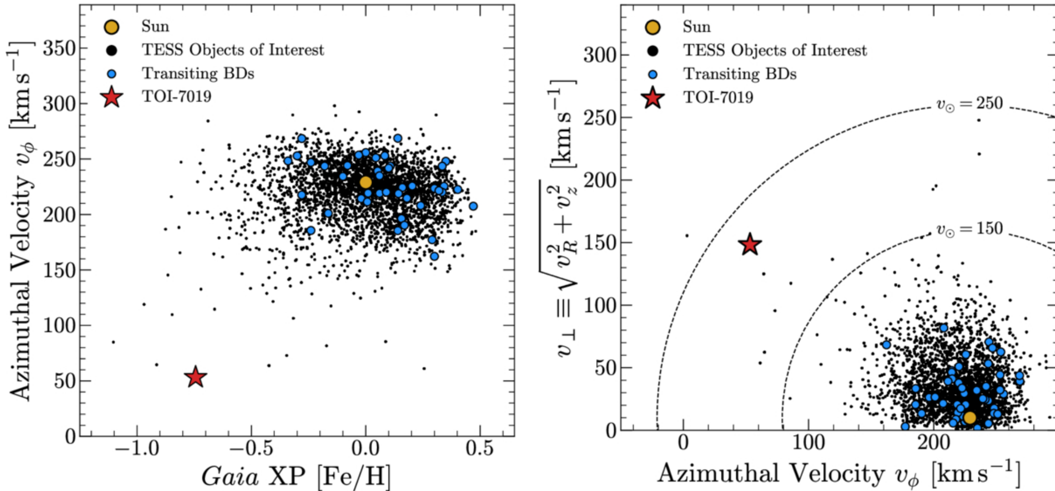
Figure 1. from Jéa Adams Redai et al 2026 Astrophys. J. Lett. 1002 doi:10.3847/2041-8213/ae4ec5 https://dx.doi.org/10.3847/2041-8213/ae4ec5 © 2026. The Author(s). Published by the American Astronomical Society.
