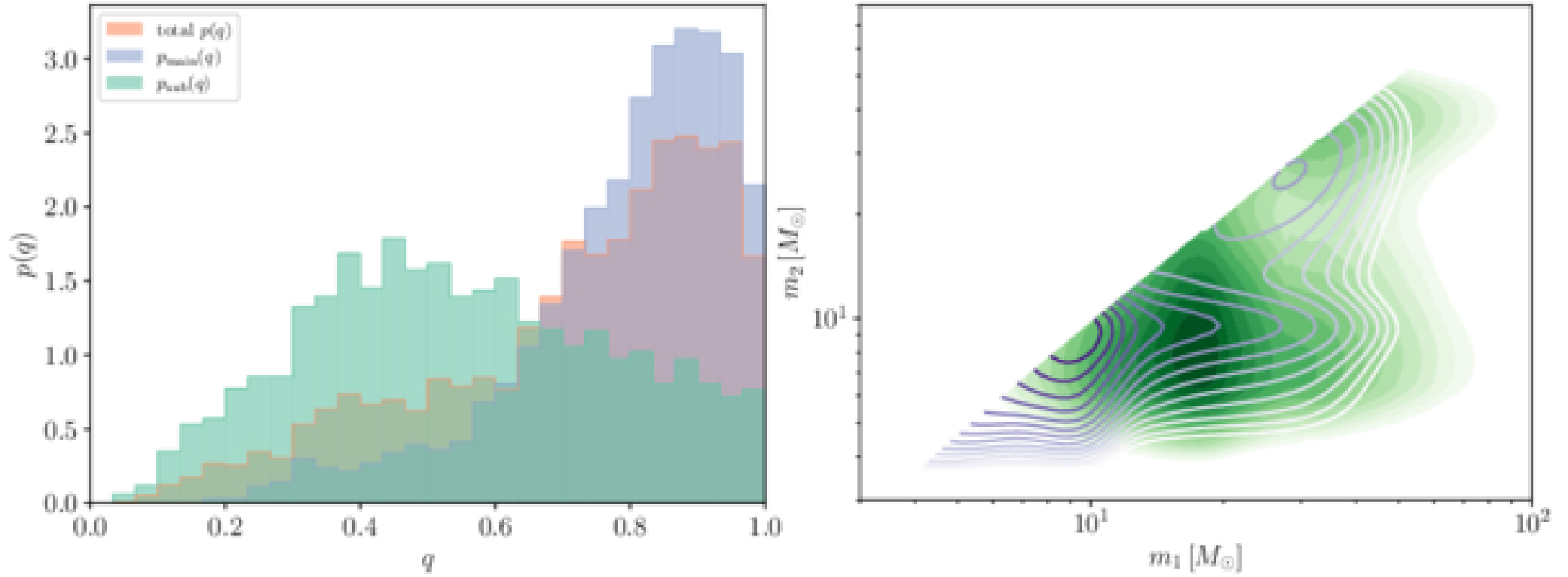
Figure 9. from Amanda M. Farah et al 2026 Astrophys. J. Lett. 1001 doi:10.3847/2041-8213/ae4e19 https://dx.doi.org/10.3847/2041-8213/ae4e19 © 2026. The Author(s). Published by the American Astronomical Society.
