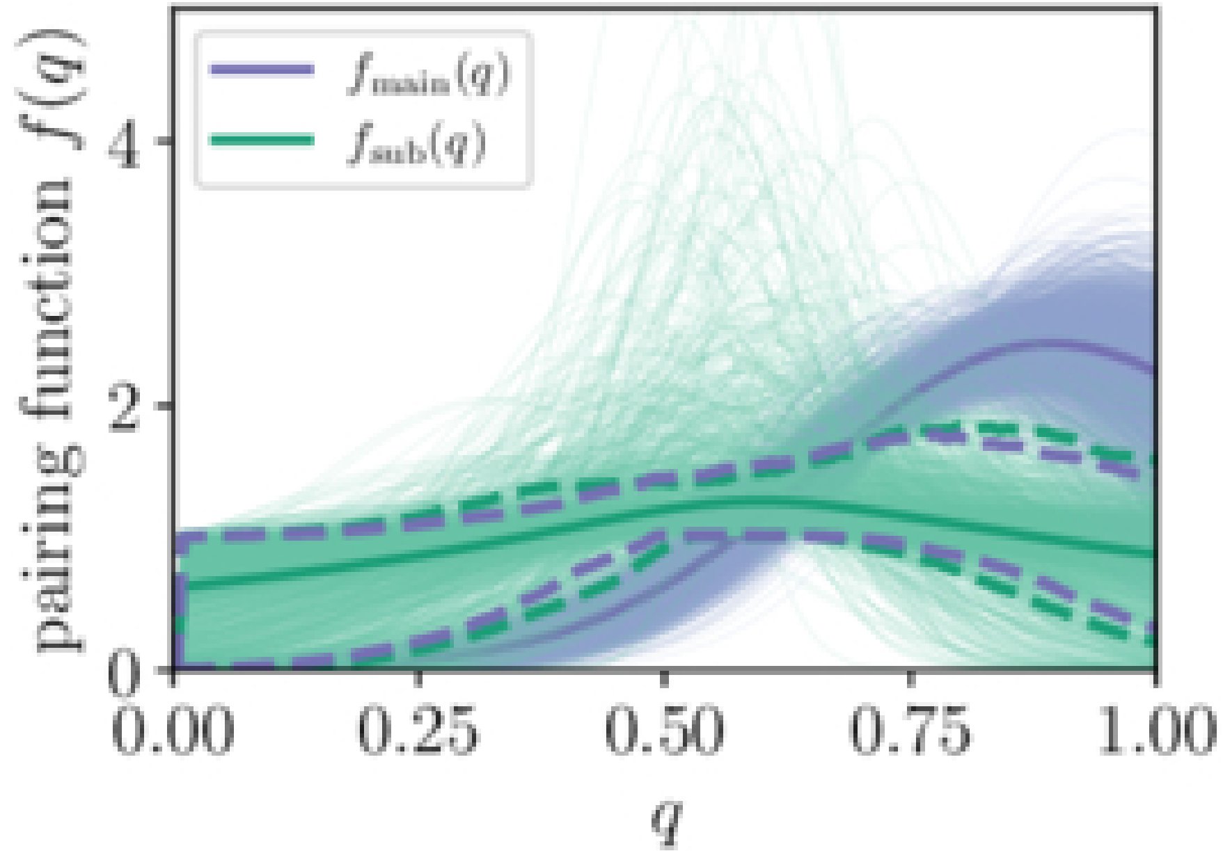
Figure 8. from Amanda M. Farah et al 2026 Astrophys. J. Lett. 1001 doi:10.3847/2041-8213/ae4e19 https://dx.doi.org/10.3847/2041-8213/ae4e19 © 2026. The Author(s). Published by the American Astronomical Society.
