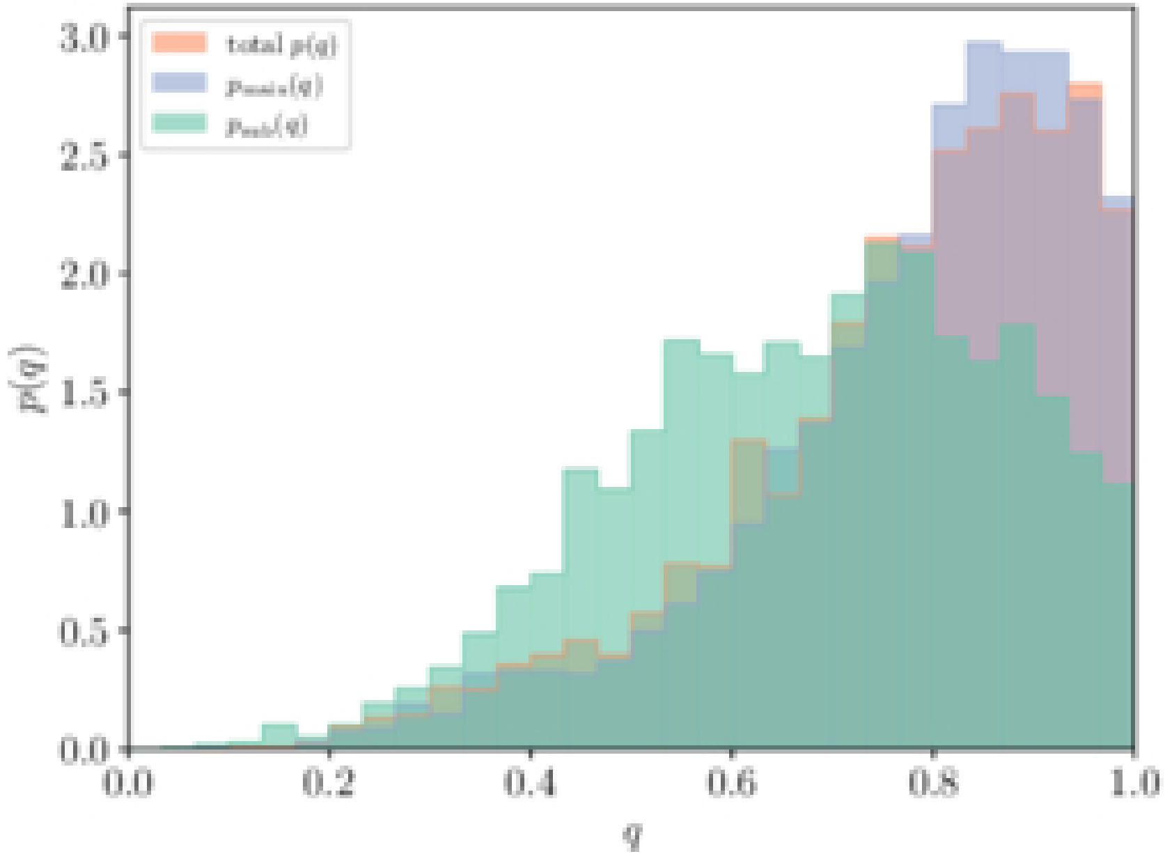
Figure 7. from Amanda M. Farah et al 2026 Astrophys. J. Lett. 1001 doi:10.3847/2041-8213/ae4e19 https://dx.doi.org/10.3847/2041-8213/ae4e19 © 2026. The Author(s). Published by the American Astronomical Society.
