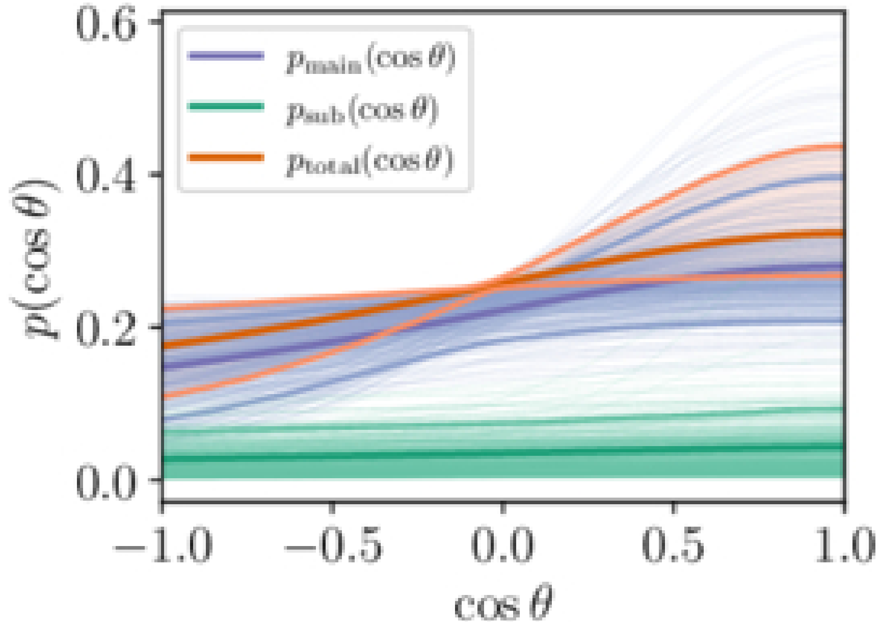
Figure 5. from Amanda M. Farah et al 2026 Astrophys. J. Lett. 1001 doi:10.3847/2041-8213/ae4e19 https://dx.doi.org/10.3847/2041-8213/ae4e19 © 2026. The Author(s). Published by the American Astronomical Society.
