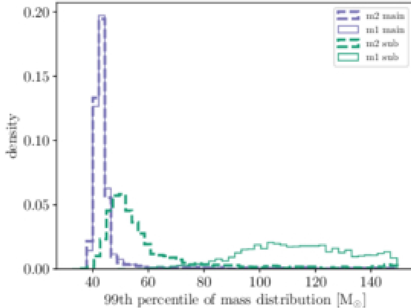
Figure 12. from Amanda M. Farah et al 2026 Astrophys. J. Lett. 1001 doi:10.3847/2041-8213/ae4e19 https://dx.doi.org/10.3847/2041-8213/ae4e19 © 2026. The Author(s). Published by the American Astronomical Society.
