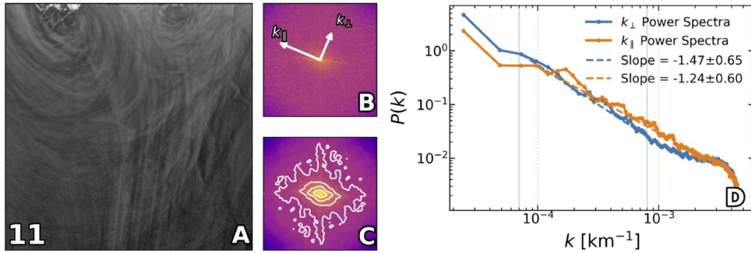
Figure 2. from Zachary Bailey et al 2026 Astrophys. J. Lett. 1002 doi:10.3847/2041-8213/ae4d16 https://dx.doi.org/10.3847/2041-8213/ae4d16 © 2026. The Author(s). Published by the American Astronomical Society.
