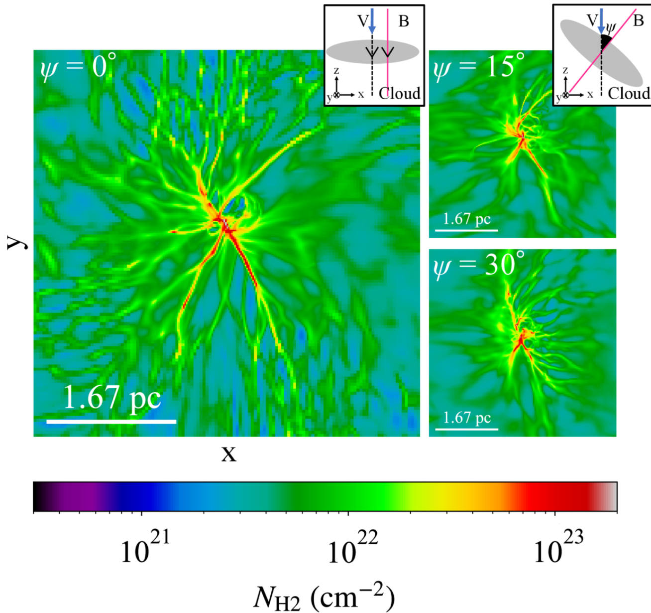
Figure 1. from Shingo Nozaki and Shu-ichiro Inutsuka 2026 Astrophys. J. Lett. 1000 doi:10.3847/2041-8213/ae4c84 https://dx.doi.org/10.3847/2041-8213/ae4c84 © 2026. The Author(s). Published by the American Astronomical Society.
