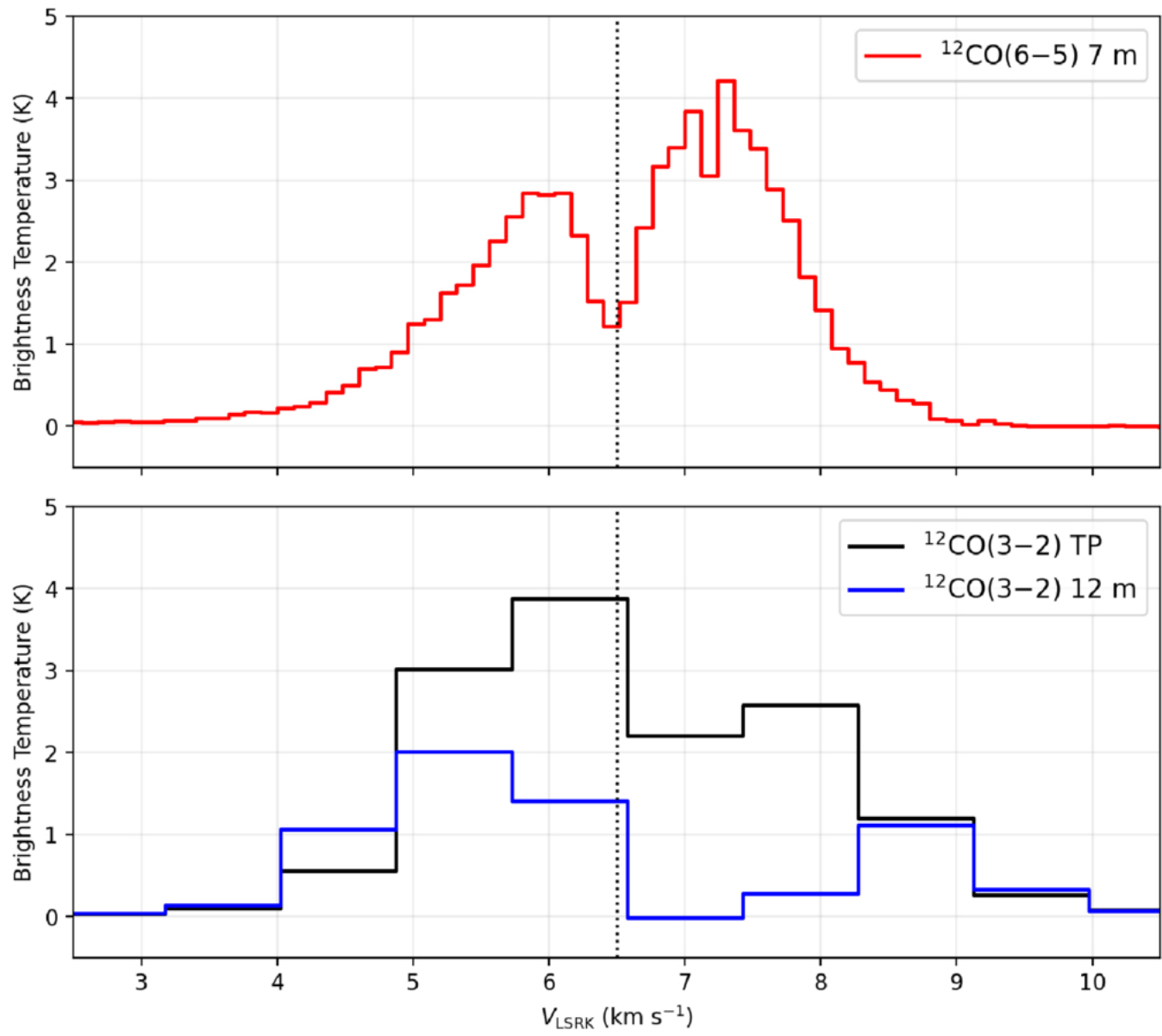
Figure 1. from Kazuki Tokuda et al 2026 Astrophys. J. Lett. 1001 doi:10.3847/2041-8213/ae47ec https://dx.doi.org/10.3847/2041-8213/ae47ec © 2026. The Author(s). Published by the American Astronomical Society.
