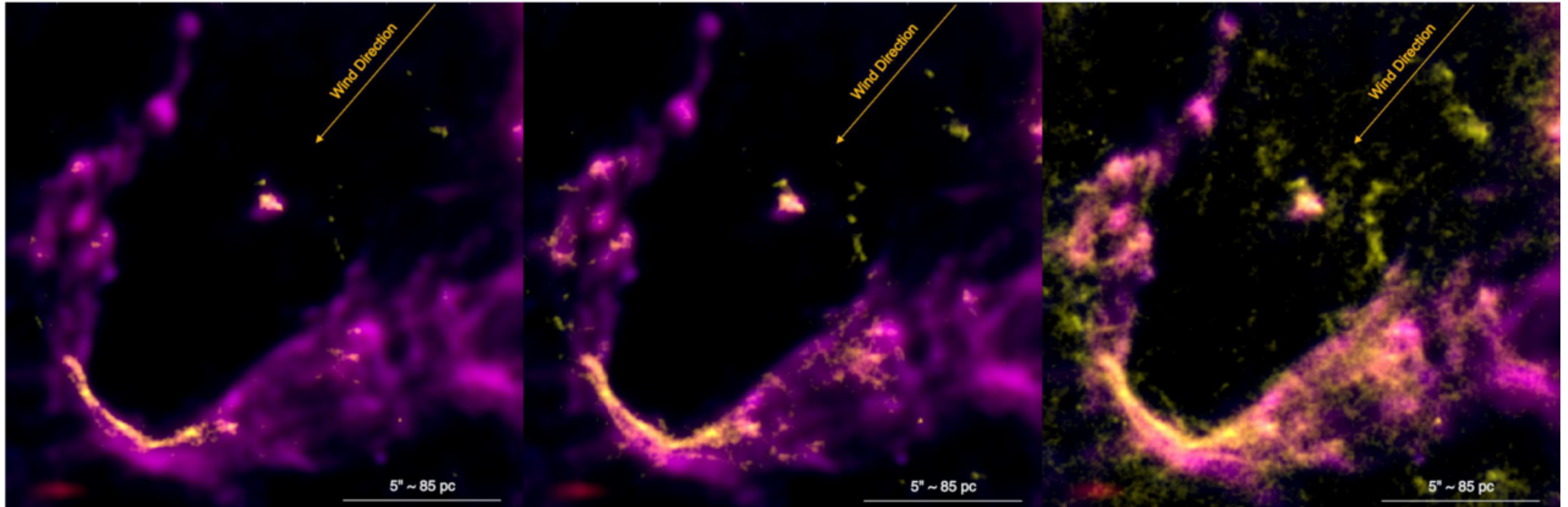
Figure B1. from Sebastian Lopez et al 2026 Astrophys. J. Lett. 999 doi:10.3847/2041-8213/ae4508 https://dx.doi.org/10.3847/2041-8213/ae4508 © 2026. The Author(s). Published by the American Astronomical Society.
