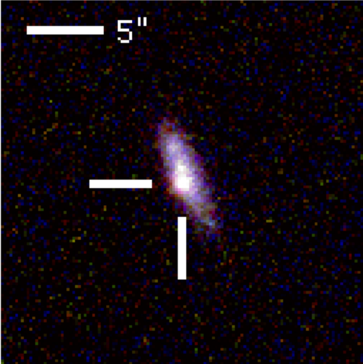
Figure 1. from Xander J. Hall et al 2026 Astrophys. J. Lett. 1001 doi:10.3847/2041-8213/ae4338 https://dx.doi.org/10.3847/2041-8213/ae4338 © 2026. The Author(s). Published by the American Astronomical Society.
