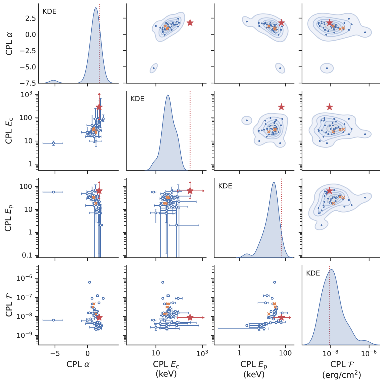
Figure 5. from Wang-Chen Xue et al 2026 Astrophys. J. Lett. 998 doi:10.3847/2041-8213/ae422b https://dx.doi.org/10.3847/2041-8213/ae422b © 2026. The Author(s). Published by the American Astronomical Society.
