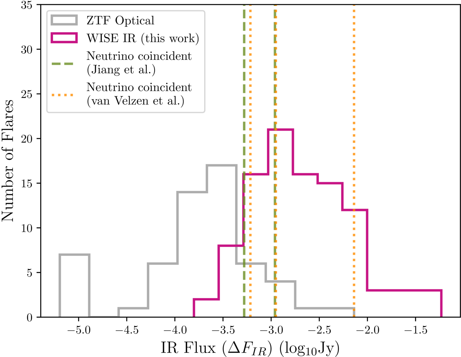
Figure 3. from Megan Wang et al 2026 Astrophys. J. Lett. 998 doi:10.3847/2041-8213/ae3f90 https://dx.doi.org/10.3847/2041-8213/ae3f90 © 2026. The Author(s). Published by the American Astronomical Society.
