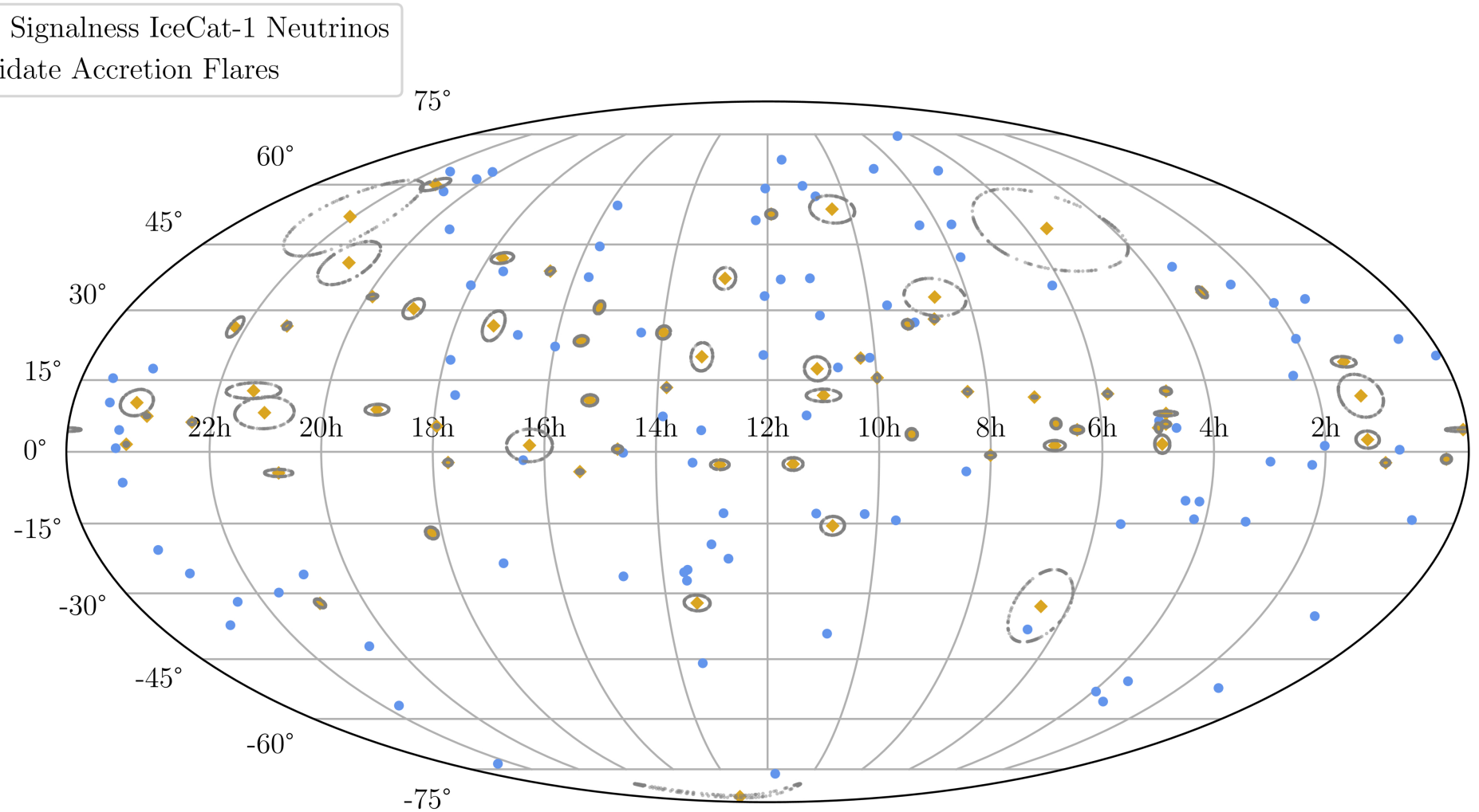
Figure 2. from Megan Wang et al 2026 Astrophys. J. Lett. 998 doi:10.3847/2041-8213/ae3f90 https://dx.doi.org/10.3847/2041-8213/ae3f90 © 2026. The Author(s). Published by the American Astronomical Society.
