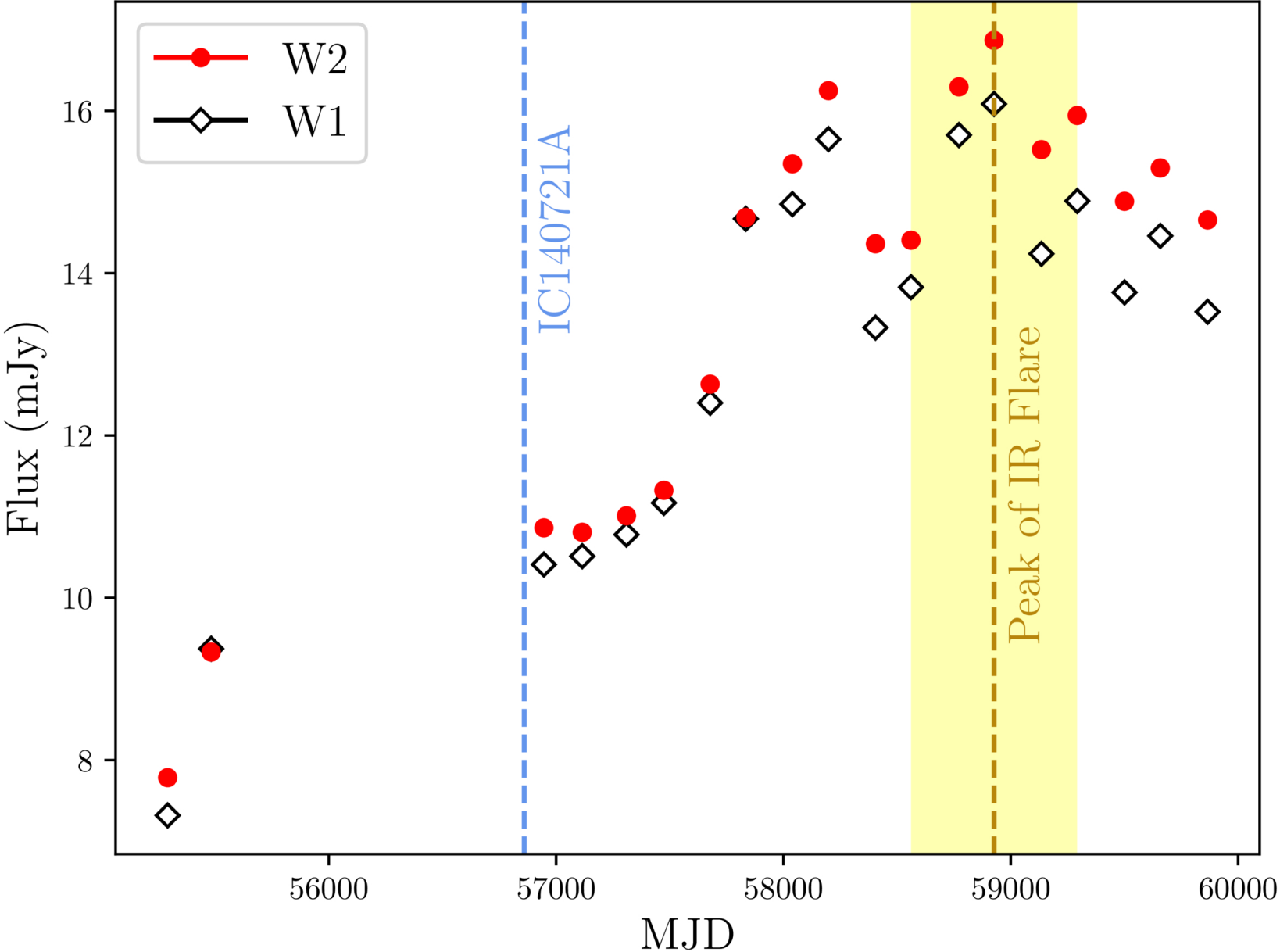
Figure 1. from Megan Wang et al 2026 Astrophys. J. Lett. 998 doi:10.3847/2041-8213/ae3f90 https://dx.doi.org/10.3847/2041-8213/ae3f90 © 2026. The Author(s). Published by the American Astronomical Society.
