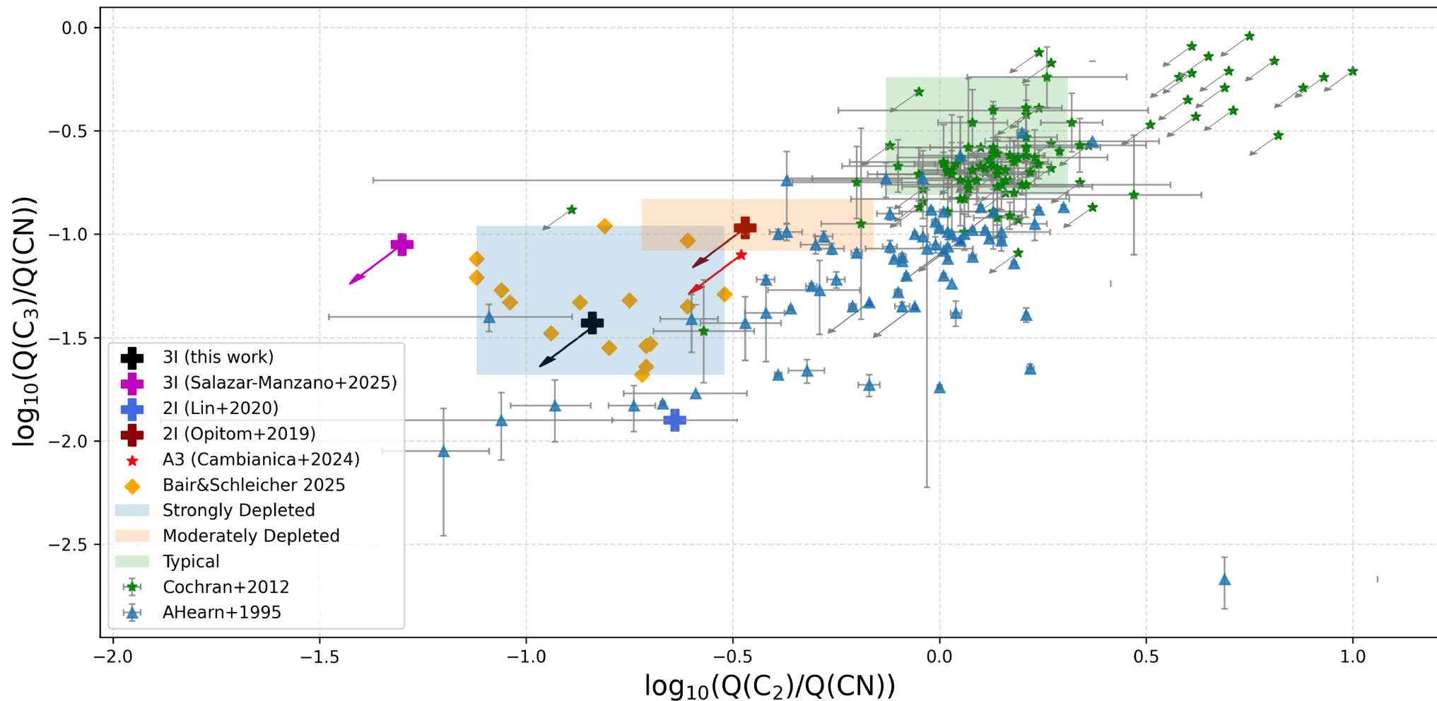
Figure 3. from M. Lazzarin et al 2026 Astrophys. J. Lett. 998 doi:10.3847/2041-8213/ae3dd7 https://dx.doi.org/10.3847/2041-8213/ae3dd7 © 2026. The Author(s). Published by the American Astronomical Society.
