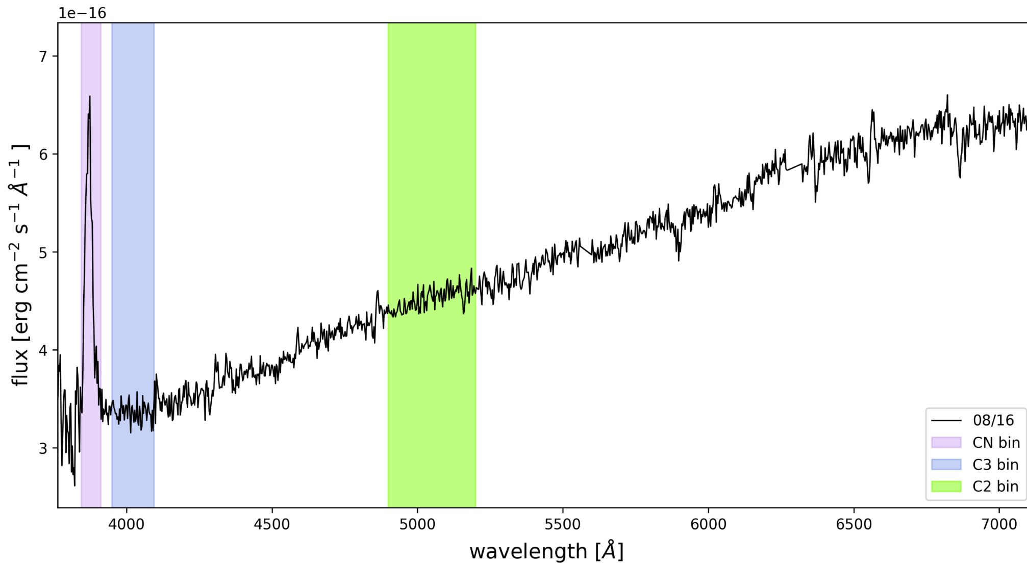
Figure 1. from M. Lazzarin et al 2026 Astrophys. J. Lett. 998 doi:10.3847/2041-8213/ae3dd7 https://dx.doi.org/10.3847/2041-8213/ae3dd7 © 2026. The Author(s). Published by the American Astronomical Society.
