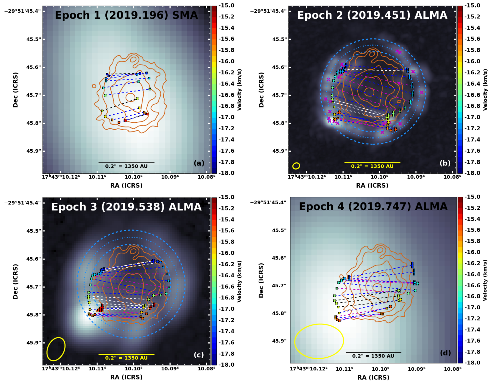
Figure 2. from T. R. Hunter et al 2026 Astrophys. J. Lett. 997 doi:10.3847/2041-8213/ae32f6 https://dx.doi.org/10.3847/2041-8213/ae32f6 © 2026. The Author(s). Published by the American Astronomical Society.
